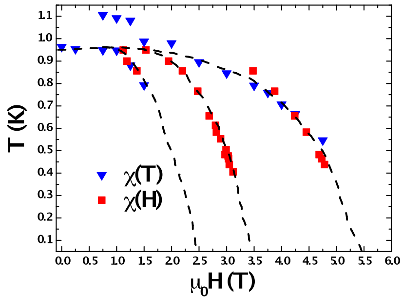
Figure 5 –Phase diagram of \text{Gd}_2\text{Sn}_2\text{O}_7 . Triangles and squares symbols denote the positions of anomalies in the ac susceptibility measured as a function of temperature and magnetic field, respectively. The lines are guide to the eyes.
