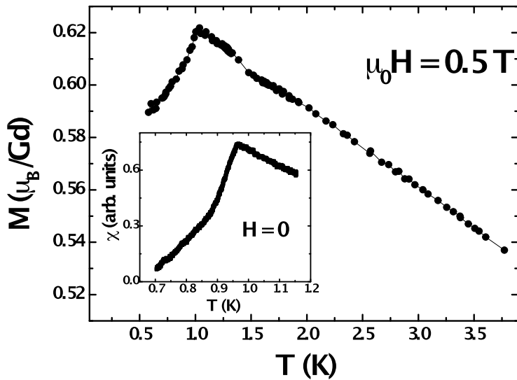
Figure 1 – Temperature dependence of the magnetization of \text{Gd}_2\text{Sn}_2\text{O}_7 measured in an applied field of \mu_0 H = 0.5 T. The inset shows the ac susceptibility as a function of temperature measured with modulation field \mu_0 h_{ac} = 1 mT and H = 0 T.
