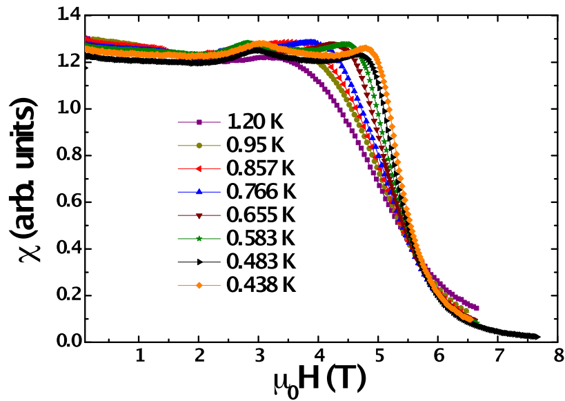
Figure 3 – Field dependence of ac susceptibility for \text{Gd}_2\text{Sn}_2\text{O}_7 at selected temperatures.
