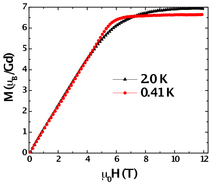
Figure 2 – Magnetization as a function of field of \text{Gd}_2\text{Sn}_2\text{O}_7 at T = 2 K and T = 0.41 K up to applied fields of \mu_0 H = 12 T.
