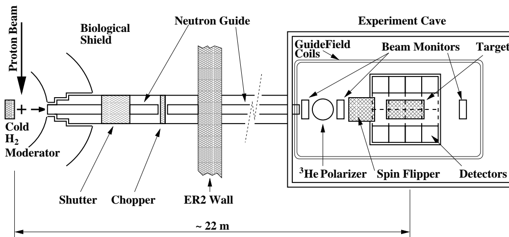
FIG. 1: Schematic of flight path 12 and the experimental setup of the NPDGamma experiment at LANSCE.
