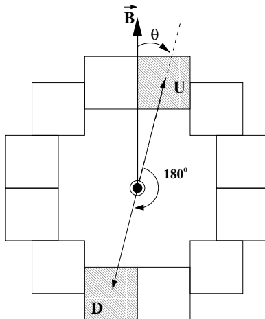
FIG. 4: A ring of 12 detectors and one up-down pair, as seen with beam direction into the page. \vec{B} is the magnetic holding field defining the direction of the neutron polarization.
