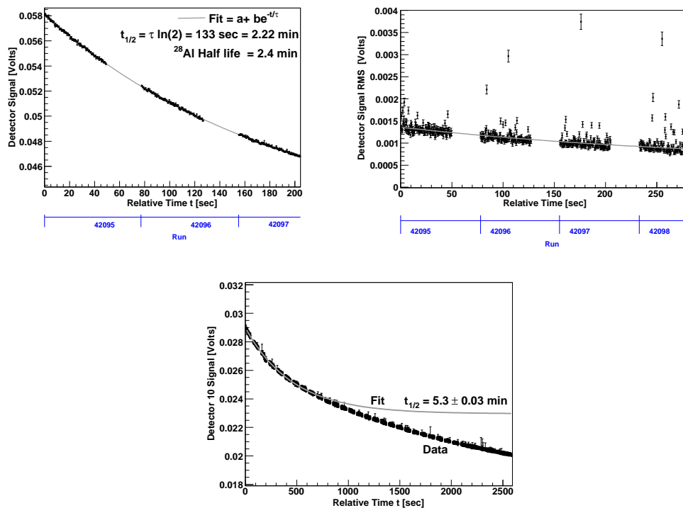
FIG. 5: Top left: Decay of pedestal mean immediately after shutter close (beam-off), showing only ^{28}\text{Al} activation. Top right: Pedestal RMS decay width. Bottom: Decay of pedestal mean, from runs taken longer after shutter closure, indicates a more complicated activation, resulting in a smaller signal with a longer half-life. The steady state pedestal levels were roughly between 20 and 40 mV depending on the detector.
