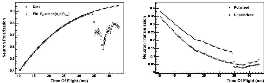
FIG. 3: Left: Plot of beam polarization as a function of neutron time of flight. Right: Neutron transmission data for an unpolarized 3 He spin filter cell and a polarized cell. The chopper cutoff is completed just below 35 ms time of flight.
