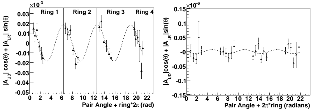
FIG. 8: Left: Measured ^{35}\text{Cl} asymmetries for each pair, plotted versus angle of the first detector in the pair with respect to the vertical. The final asymmetry is extracted from the fit A_{UD}\cos(\theta) + A_{LR}\sin\theta , with A_{UD} and A_{LR} as fit parameters. Right: Asymmetries from noise measurements.
