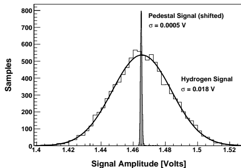
FIG. 6: \gamma -ray counting statistics analysis for a typical detector module. The RMS width for beam-on signal is compared to the width seen from pedestal runs. A fit to the beam on data histogram with LH 2 target shows an RMS width of 18.4 \pm 0.13 mV.
