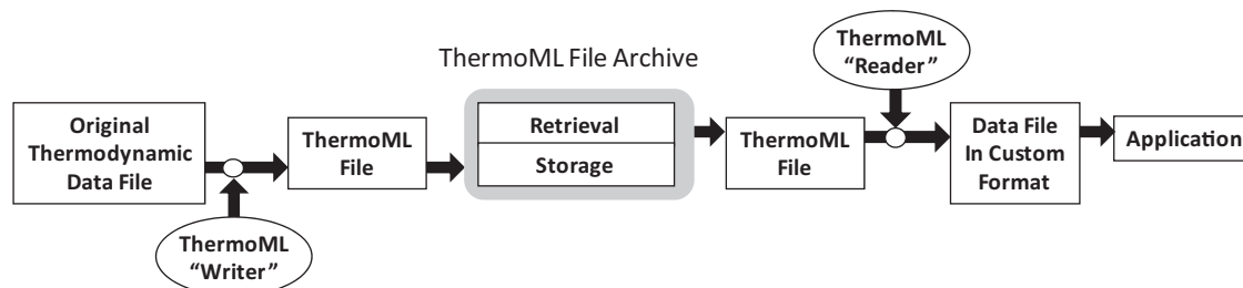
Fig. 2. Global delivery process for experimental thermophysical and thermochemical property data.
