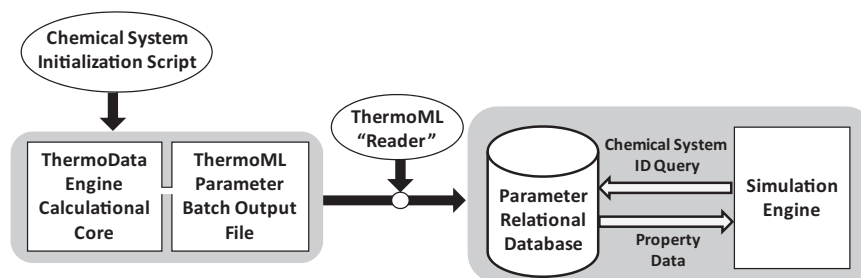
Fig. 4. Implementation of the ThermoML information “bridge” for a family of chemical systems in a batch mode.
