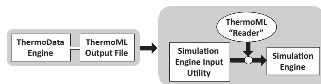
Fig. 3. Implementation of the ThermoML information “bridge” for a single chemical system.
