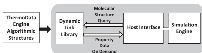
Fig. 5. Implementation of the information “bridge” based on dynamic link library (DLL) technology.
