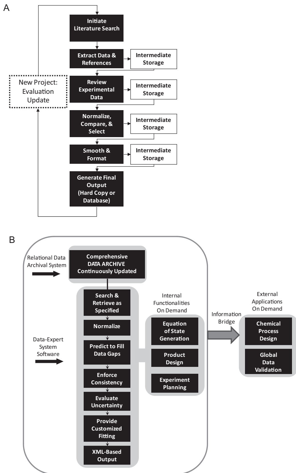
Fig. 1. (A) Schematic representation of static data evaluation performed by an evaluator in advance of use. (B) Schematic representation of dynamic data evaluation performed by a user on demand.
