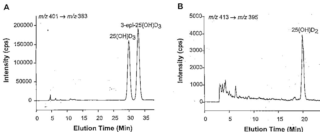
Figure 2. LC-MS/MS multiple reaction monitoring chromatograms for Level 4 of SRM 972. Measurements of 25(OH)D 3 and 3-epi-25(OH)D 3 were made using a Zorbax CN column (A) and measurements of 25(OH)D 2 were made using a Zorbax XDB-C 18 column (B). Further experimental details are provided in the text.
