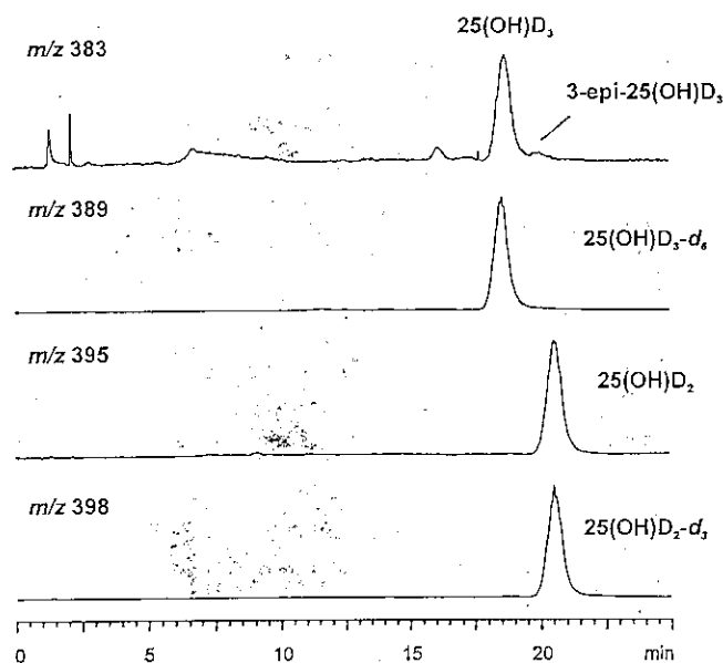
Figure 1. Selected ion chromatograms (LC-MS) for vitamin D metabolites and their labeled internal standards in Level 3 of SRM 972. Experimental details are provided in the text.
