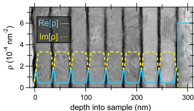
FIG. 3. (Color online) Nuclear composition used to fit the PNR data at all T . Gd is evident by decreased \text{Re}\{\rho\} and increased \text{Im}\{\rho\} . The background is a scaled cross-sectional TEM image.
