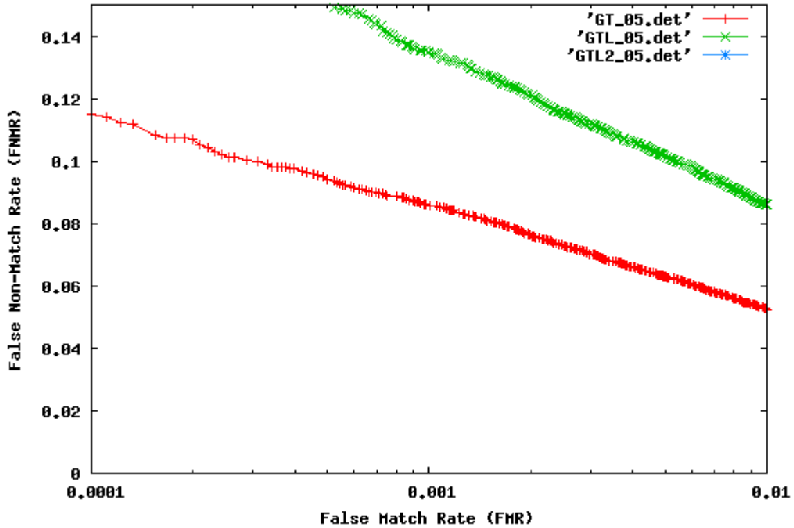
Hand Marked - Single Finger Results (05) for Matcher I
