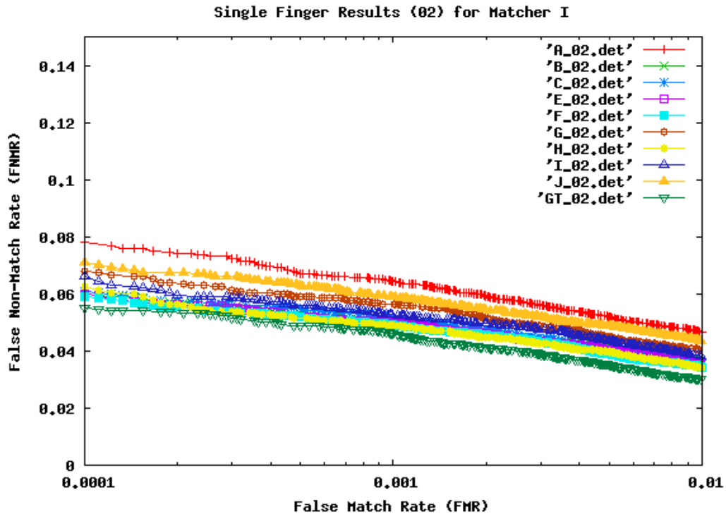
Figure 1: DET - Matcher-I – Finger 02 – Segmentation Algorithm Boxes.
