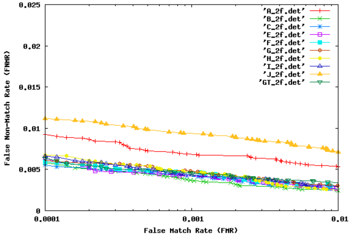
Two Finger Results for Matcher III
