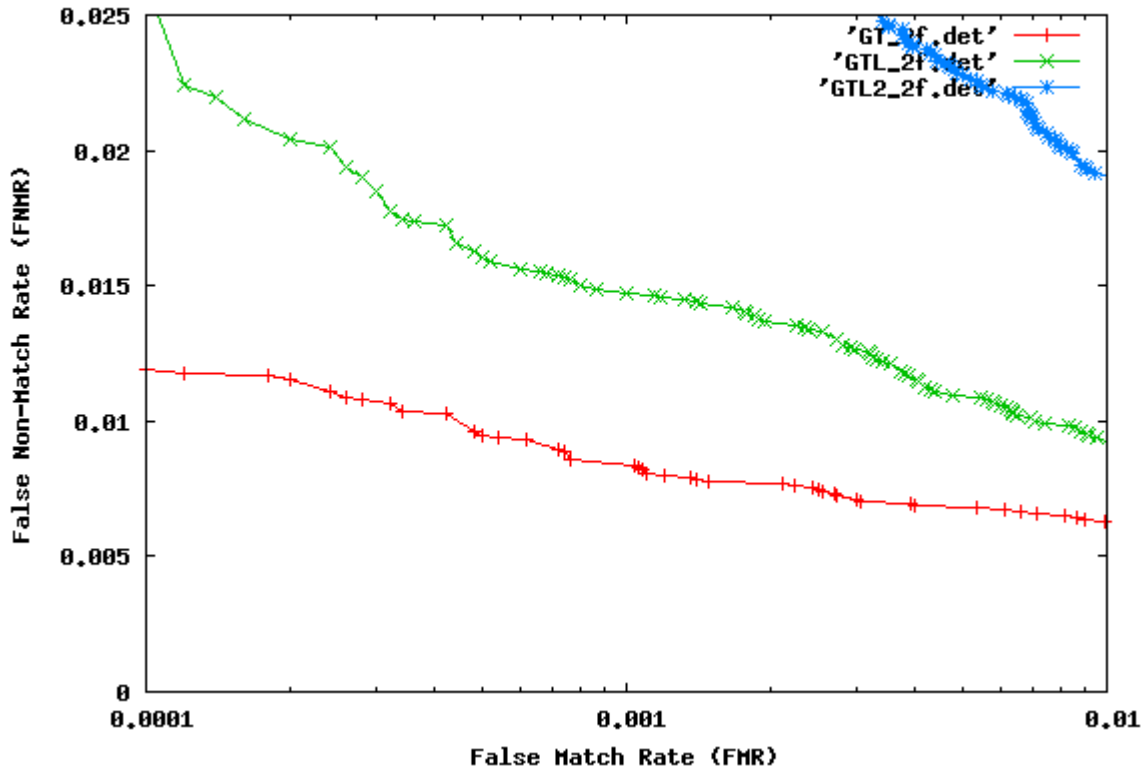
Hand Marked - Two Finger Results for Matcher II
