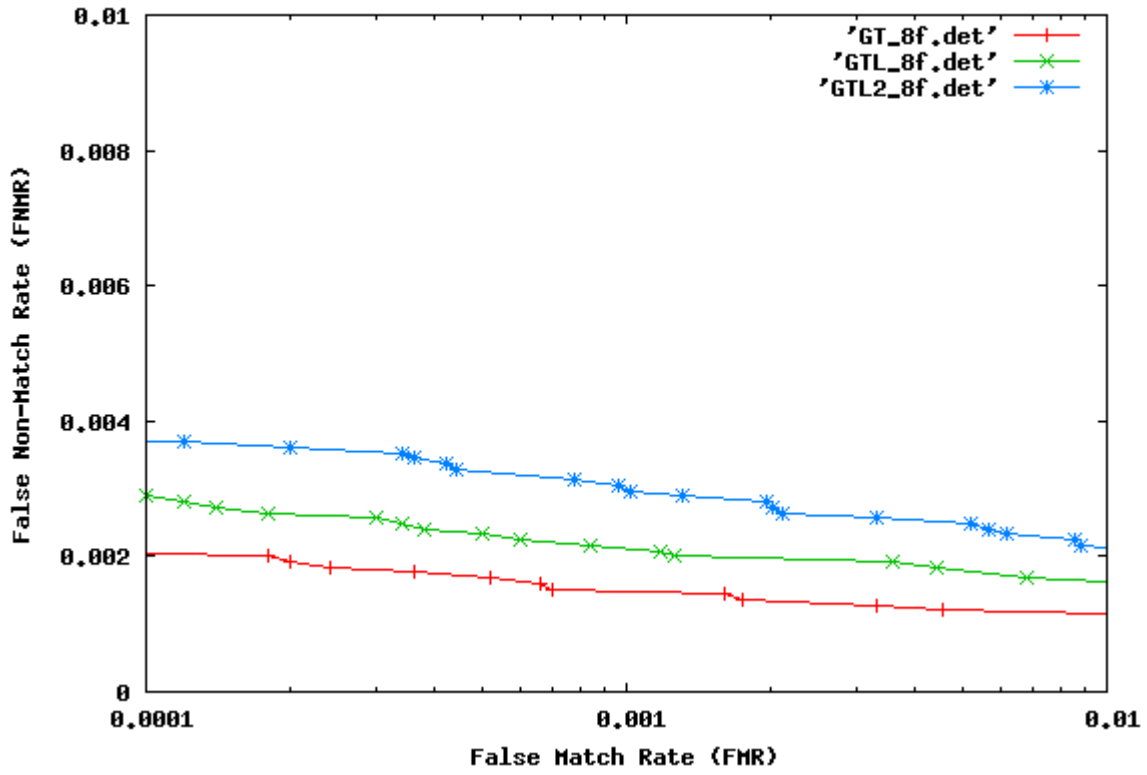
Hand Marked - Eight Finger Results for Matcher III
