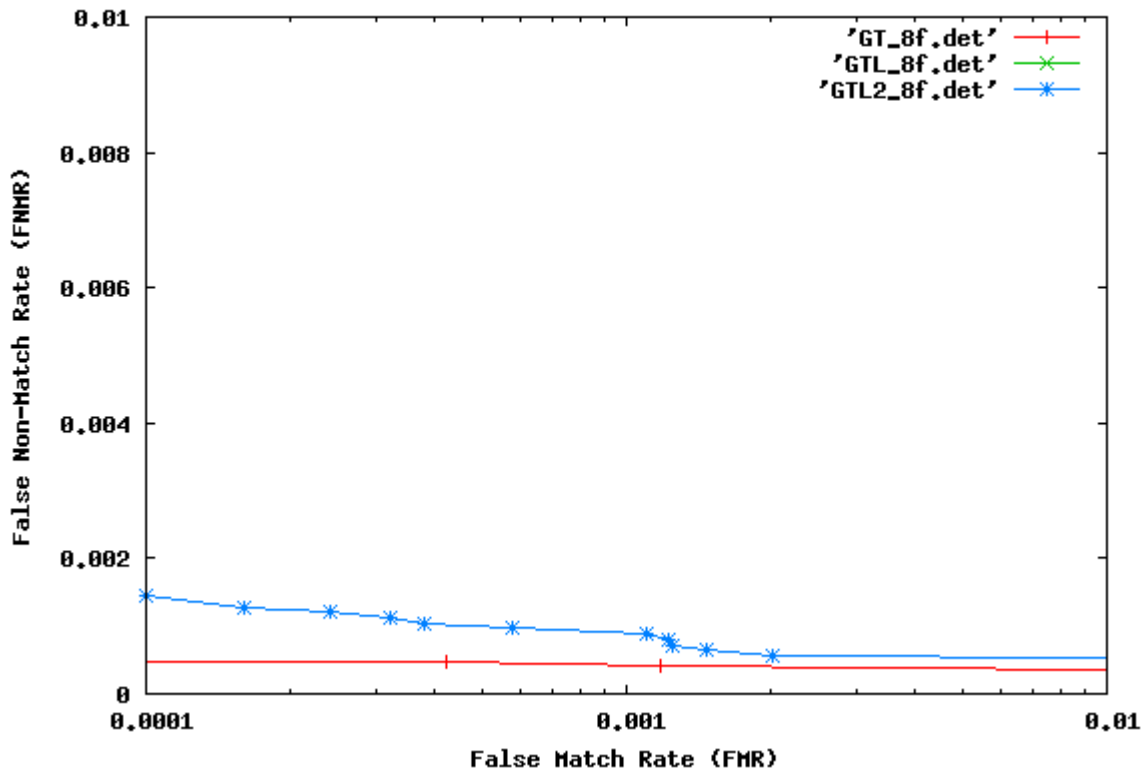
Hand Marked - Eight Finger Results for Matcher II
