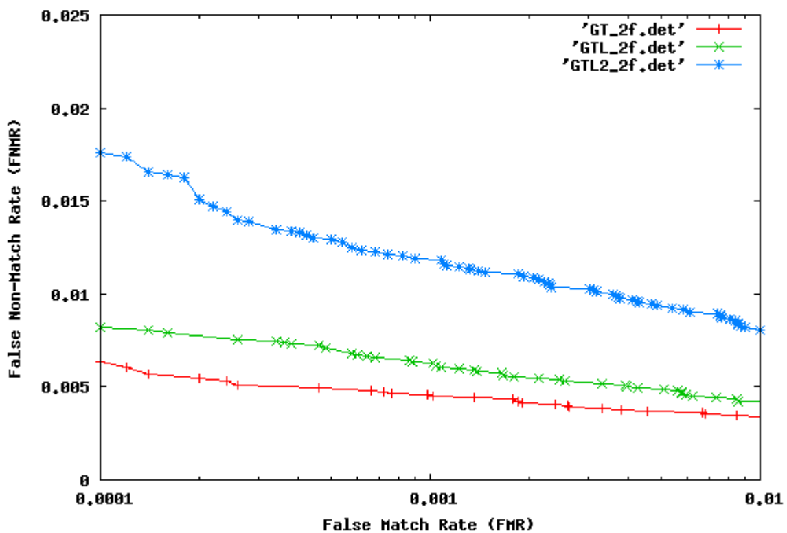
Hand Marked - Two Finger Results for Matcher III
