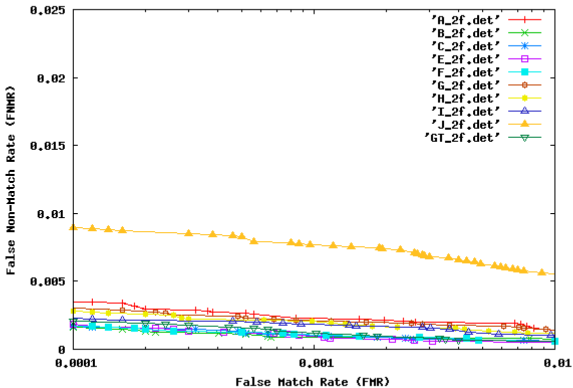
Two Finger Results for Matcher II
