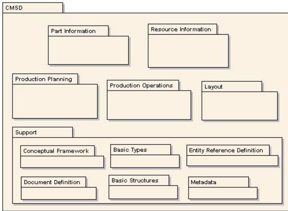
Figure 2 - CMSD Package Diagram
