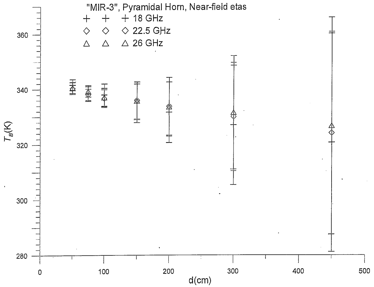
Figure 1. Measured and predicted target temperature vs. distance
