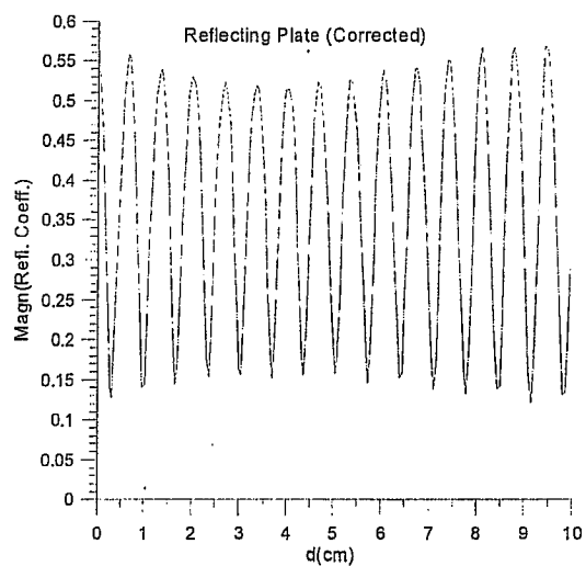
Fig. 4 Results for aluminum plate.
