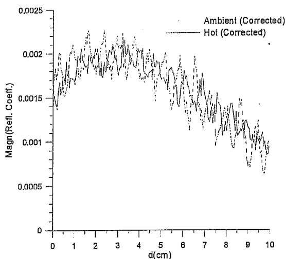
Fig. 3 Comparison of hot and ambient targets.
