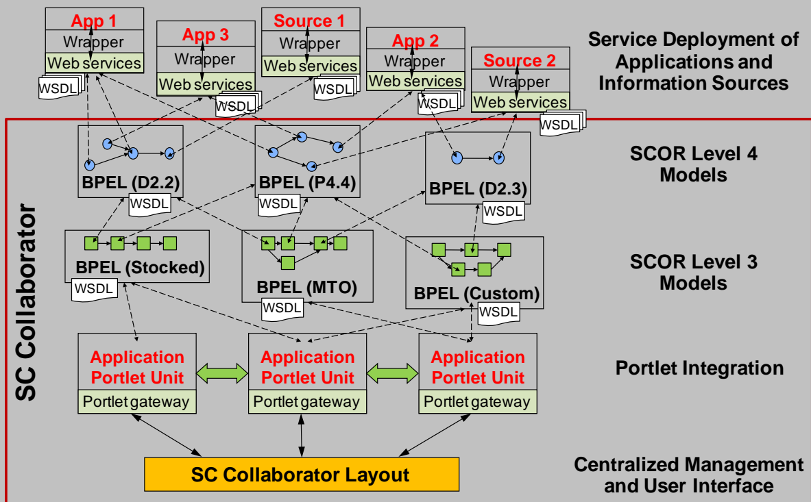
Figure 24: Incorporating SCOR Level 3 and Level 4 models in SC Collaborator
