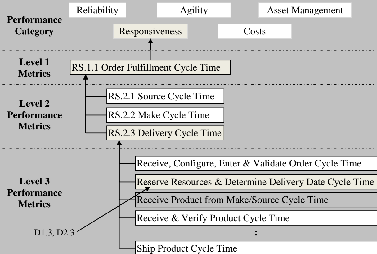
Figure 20: Performance metrics hierarchically structured in the SCOR guidelines
