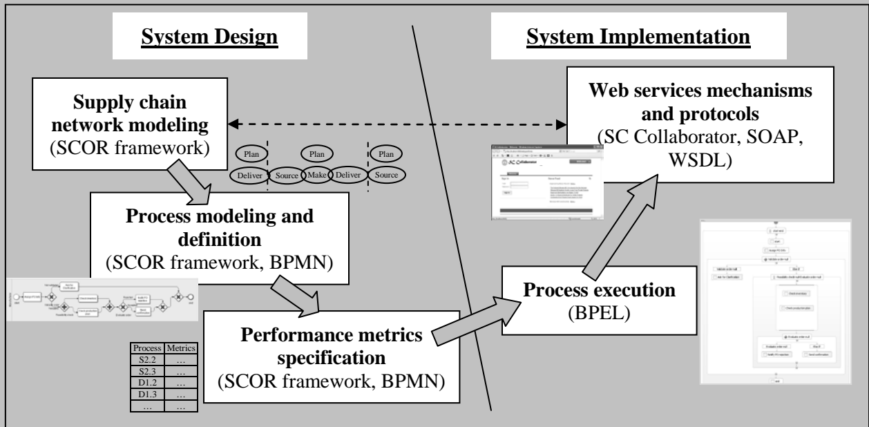
Figure 19: Development framework for service oriented supply chain performance monitoring systems using the SCOR framework, open standards, and open source technologies
