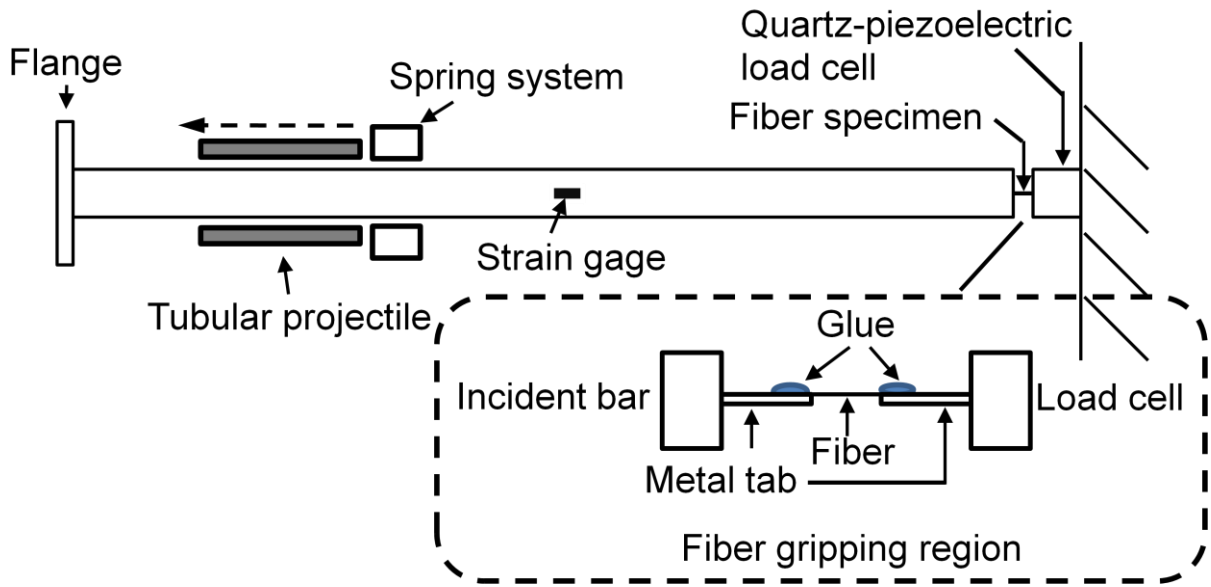
Figure 1. Schematic of the experimental setup for single fiber tensile tests using Kolsky bar.
