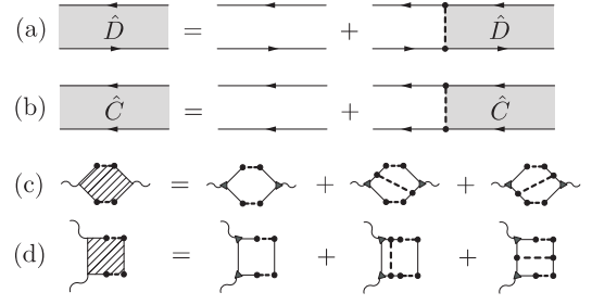
FIG. 9 (Color online) Diagrammatic representation for (a) diffuson, (b) Cooperon, and dressed Hikami boxes [(c) and (d)]. Figure adapted from Kharitonov and Efetov (2008)
