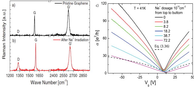
FIG. 25 (Color online) Left panel: Raman spectra (wavelength 633 nm) for (a) pristine graphene and (b) graphene irradiated by 500 eV \text{Ne}^+ ions that are known to cause vacancies in the graphene lattice. Right panel: Increasing the number of vacancies by ion irradiation caused a transition from the pristine graphene (where Coulomb scattering dominates) to the lower curves where scattering from vacancies dominate. Also shown is a fit to Eq. 3.36 from Stauber et al. (2007) that describes scattering off vacancies that have midgap states. Figures taken from Chen et al. (2009c).
