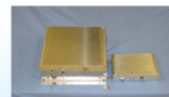
Comparison of MMFDS (10" x 10" x 4.50") to Miniaturized MultiParameter Smart Space Fire Detection System (7.00" x 5.85" x 2.12")
