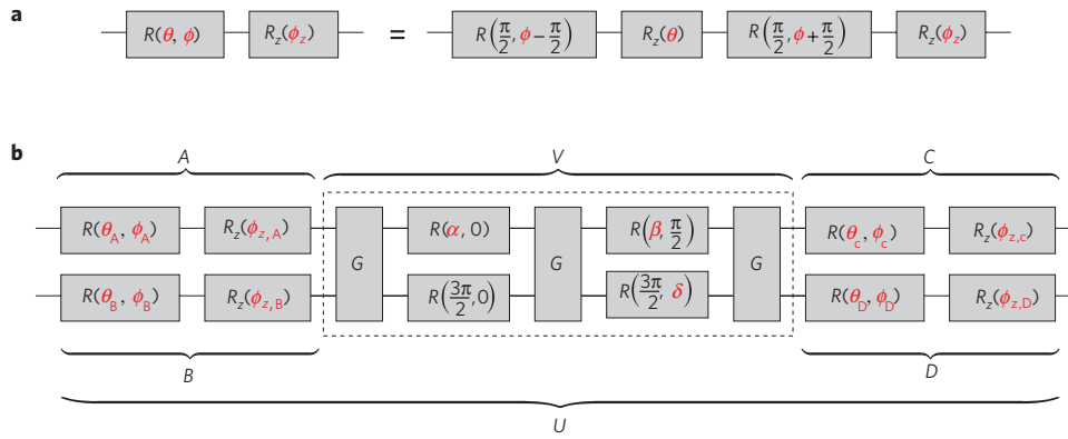
Figure 1 | Components for universal computation. a, b , Circuit diagrams for arbitrary unitary transformations on one ( a ) and two ( b ) qubits. The operations for each circuit are implemented from left to right, with each line representing one qubit. a also indicates the decomposition used for R(\theta, \phi) . The dashed rectangle in b contains the three degrees of freedom \alpha, \beta and \delta that determine the two-qubit operation's local equivalence class. The brackets highlight the decomposition of the two-qubit operation U as described in the text: U = (C \otimes D) \cdot V \cdot (A \otimes B) .
