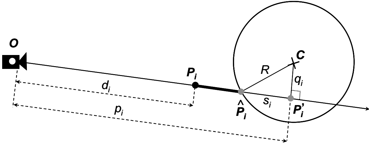
Figure 1. Geometrical interpretation of the directional error function when a scan ray intersects the sphere surface. \mathbf{P}_i (marked by dark dot) is the experimental point, light dots mark the theoretical point on the sphere surface \hat{\mathbf{P}}_i and the mid-chord point \mathbf{P}'_i . The length of the bold line segment measures the error f_i defined by (3.1.3).
