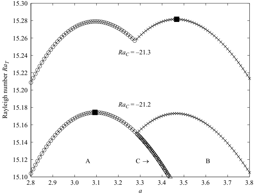
FIGURE 3. This plot shows neutral stability curves for two different values of Ra_C near the transition between real (O) and oscillatory (X) modes. The lower curves also indicate further structure of these modes and the regions with one unstable real mode (denoted by A), two unstable oscillatory modes (denoted by B) and two unstable real modes (denoted by C). The parameter values used here (corresponding to solution 4 shown in figure 2) are m_1 = m_2 = 0.5 , Le_1 = Le_2 = 100 , k_1 = k_2 = 0.1 , S = 37 , k_s/k_l = 1 , c_s/c_l = 1 , V = 0.1 , \phi_0 = 0.1 , C_1^{bot} = -3.5 , C_2^{bot} = -3 and N_p = 32 .
