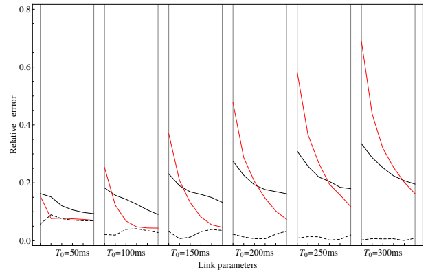
Fig. 7. Relative error for the AMS model with \alpha=1.4 (black), \alpha=4 (dashed black) and M/M/1/B (red).
