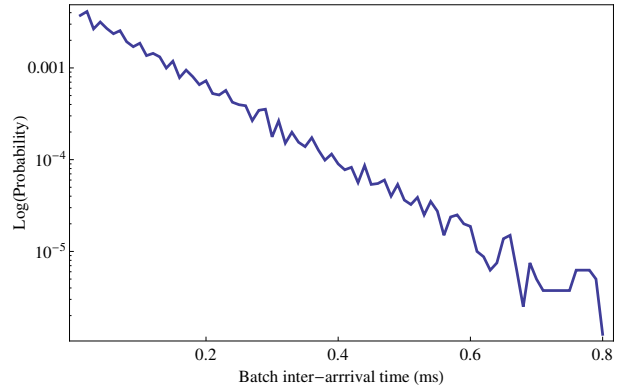
Fig. 3. Sample log probability plot of batch inter-arrival time distribution based on ns2 packet traces.
