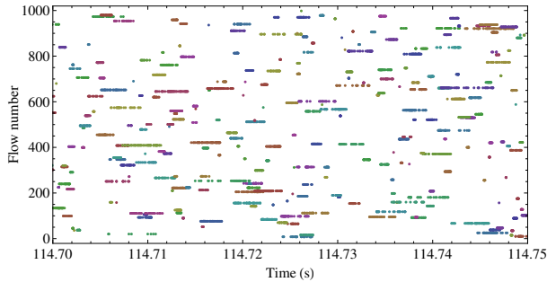
Fig. 2. Packet arrival times separated by flow number
