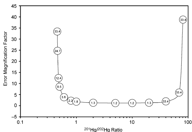
Fig. 3 Error magnification factor as a function of ^{201}\text{Hg}/^{202}\text{Hg} isotope dilution ratio.
