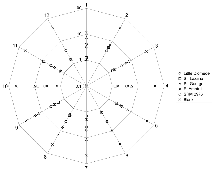
Fig. 4 Radar plot showing all measured ^{201}\text{Hg}/^{202}\text{Hg} isotope dilution ratios (log axis) for each sample batch.
