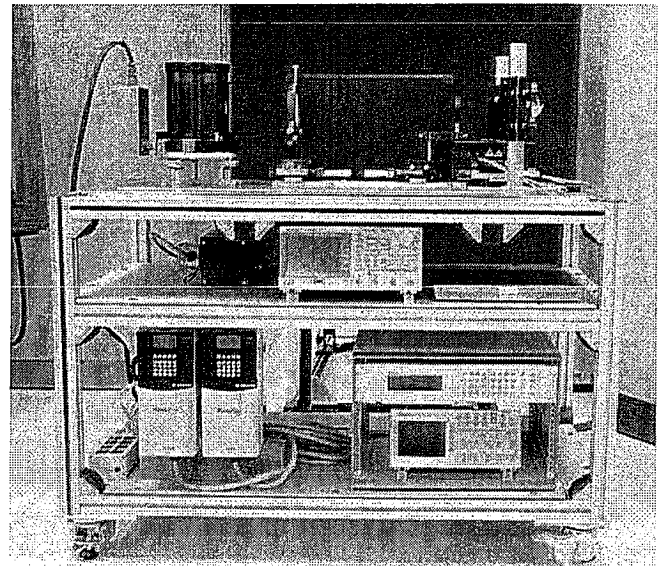
Fig. 4. Photograph of our terahertz imaging and spectroscopy system assembled on a mobile cart platform.
