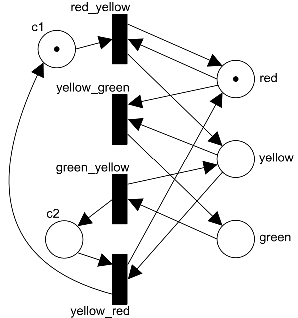
Figure 1: Petri Net for Example 1 (used by permission from Wil van der Aalst [12])
