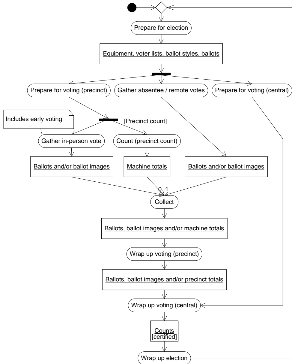
Figure 3: Activity Diagram for Example 2
