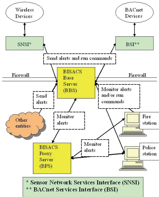
Figure 1 BISACS Architectural Overview
