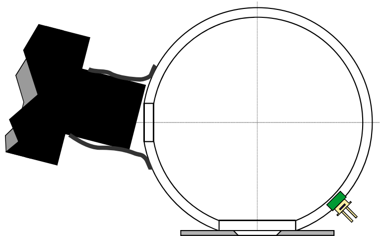
Figure 10. Horizontal cross-section of integrating-sphere detector. A photopic photodiode is embedded in the wall without destroying the interior surface. When the spectroradiometer is used, a black-felt multilayer wrap surrounds the lens and near surface of the sphere to avoid any introduction of stray light.
