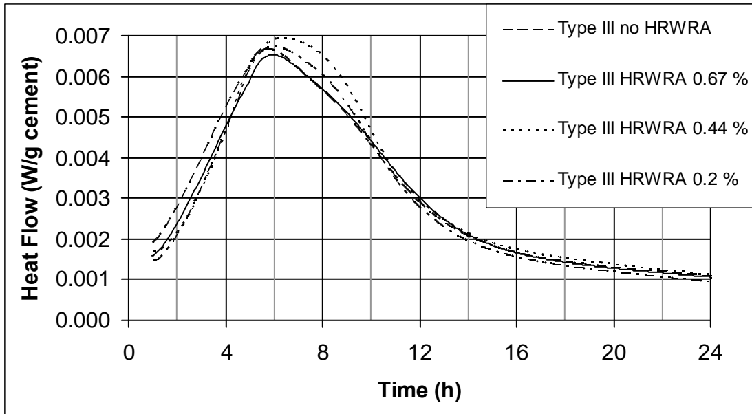
Figure 5. Isothermal calorimetry results out to 24 h for Type III w/c=0.4 cement pastes with various addition rates (by mass of cement) of HRWRA. 1 \text{ W/g} = 1548 \text{ BTU}/(\text{h}\cdot\text{lb}) .
