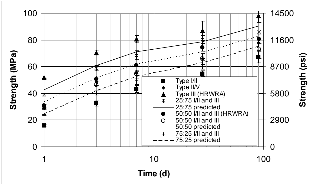
Figure 13. Measured and predicted (law of mixtures) compressive strengths vs. time for the various mortar mixtures. Error bars for each symbol indicate \pm one standard deviation for three replicate specimens for each mortar at each age.
