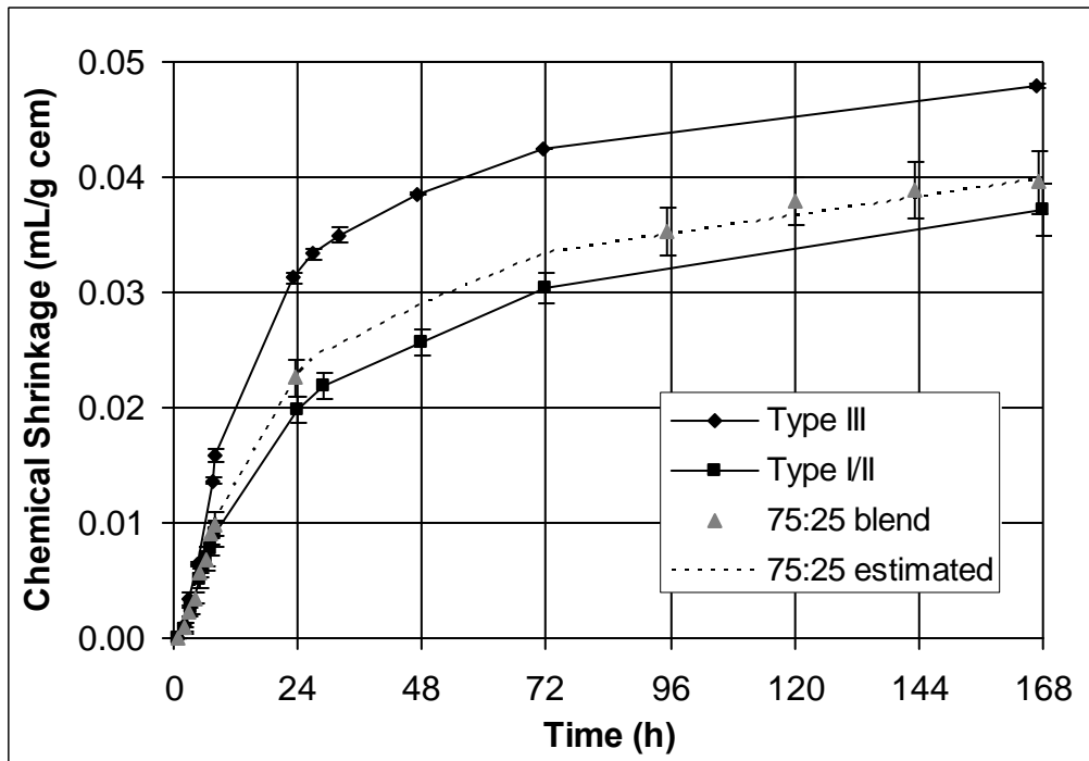
Figure 7. Chemical shrinkage results for the Type I/II and III w/c=0.4 cement pastes and results for the 75:25 w/c=0.4 blend, both as measured and as predicted by applying the law of mixtures. Error bars indicate \pm one standard deviation for three replicate specimens for each cement paste. 1 mL/g = 15.34 oz/lb.
