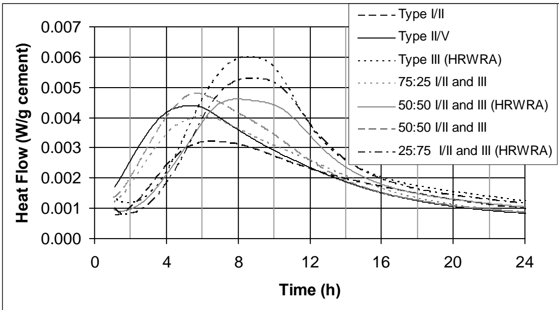
Figure 11. Isothermal calorimetry results out to 24 h for w/c=0.4 mortars based on the three initial cements and the blends of the Type I/II and Type III cements. 1 \text{ W/g} = 1548 \text{ BTU}/(\text{h}\cdot\text{lb}) .
