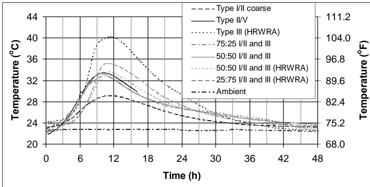
Figure 12. Semi-adiabatic temperature vs. time for mortars.
