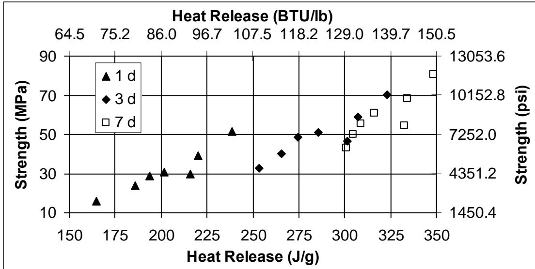
Figure 14 . Compressive strength vs. heat release at 3 different ages for the mortars examined in this study. For each age, data points from left to right correspond to Type I/II, 75:25 blend, Type II/V, 50:50 blend with HRWRA, 50:50 blend with no HRWRA, 25:75 blend, and Type III cements, respectively.
