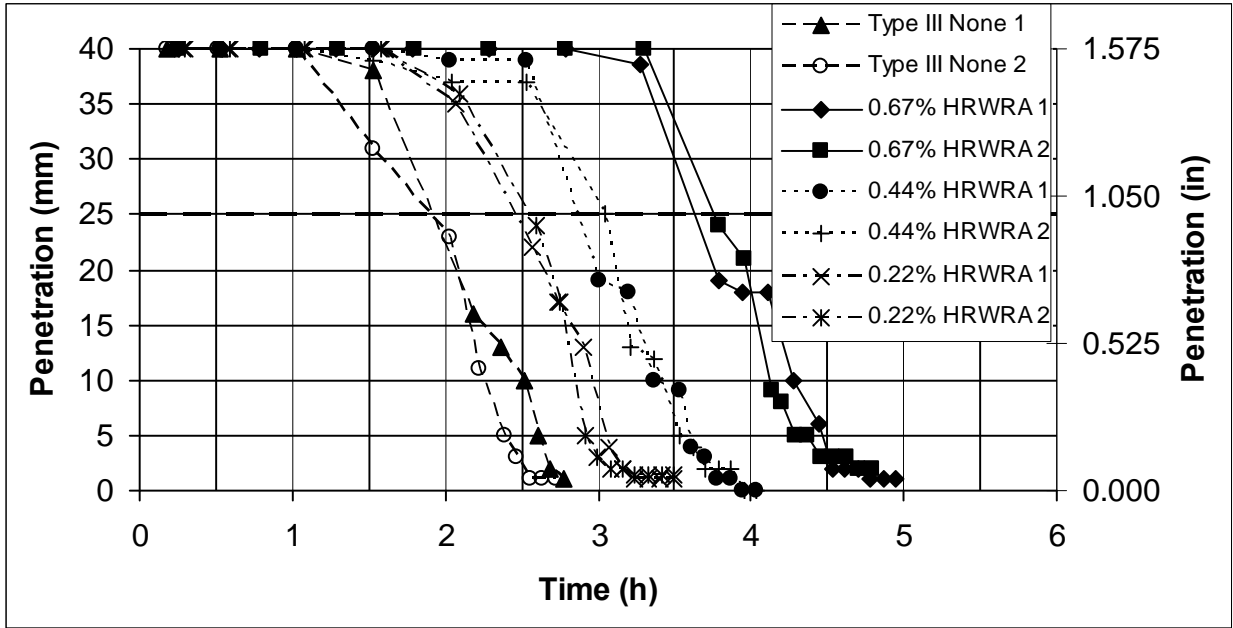
Figure 10. Setting time results for w/c=0.4 Type III cement pastes with various HRWRA addition levels. Dashed line at a penetration of 25 mm (1 in) indicates initial set. Two replicate measurements from the same batch are shown for each paste to provide an indication of variability.
