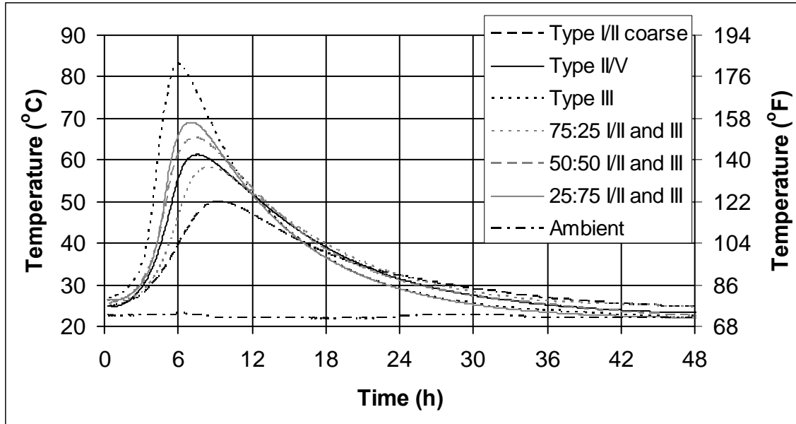
Figure 8. Semi-adiabatic temperature vs. time for the six w/c=0.4 cement pastes.
