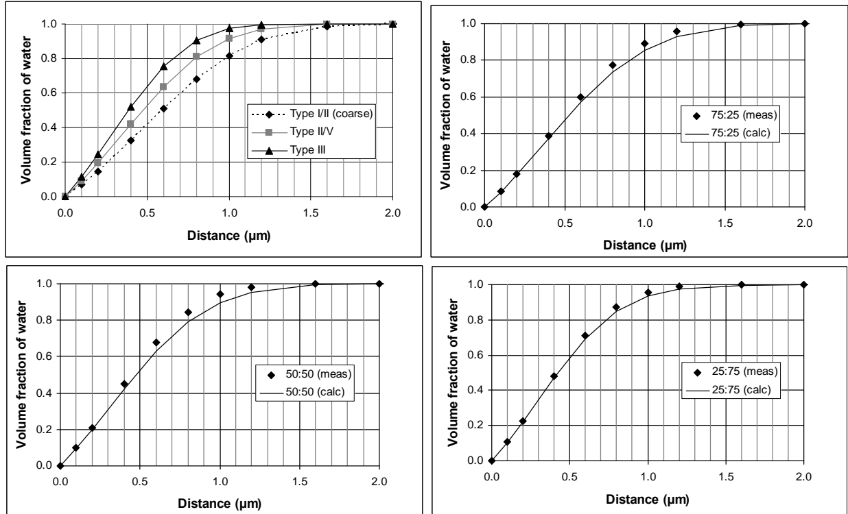
Figure 3. Volume fraction of water within a given distance of a cement particle surface for the simulated initial cement microstructures for w/c=0.4 cement pastes. (One micrometer is equivalent to 3.9 \times 10^{-5} in.)
