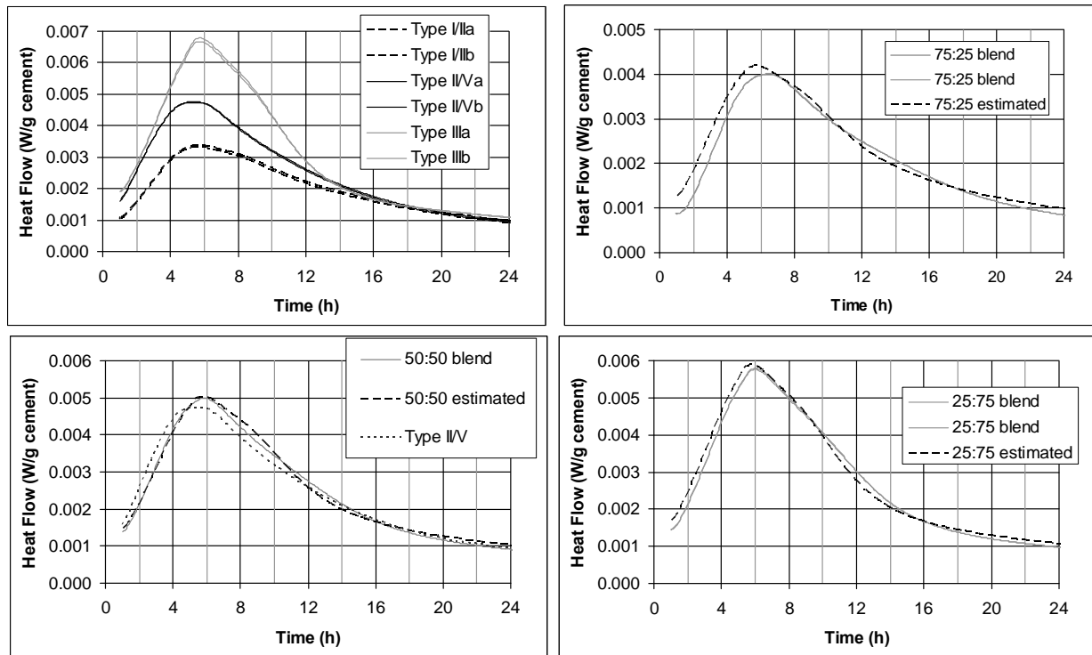
Figure 4. Isothermal calorimetry results out to 24 h for Type I/II, II/V, and III cements (top left) and for the three blends ( w/c=0.4 pastes). Results for two replicate specimens are shown for most pastes. 1 W/g = 1548 BTU/(h·lb).
