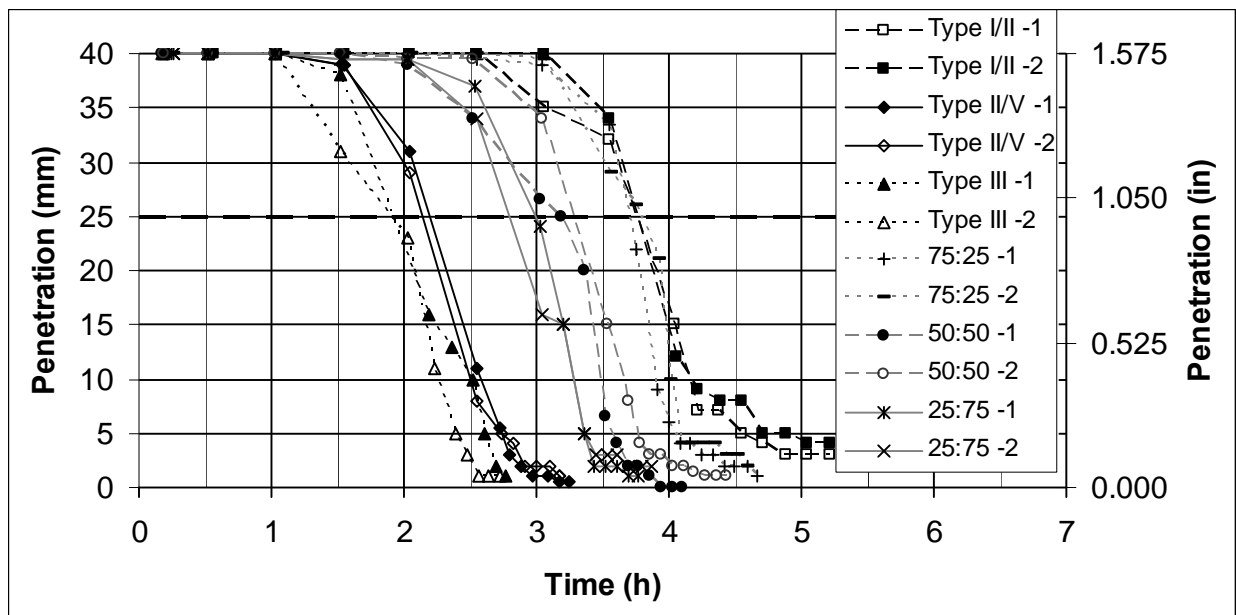
Figure 9. Setting time results for w/c=0.4 cement pastes for the three initial cements and the three blends. Dashed line at a penetration of 25 mm (1 in) indicates initial set. Two replicate measurements from the same batch are shown for each paste to provide an indication of variability.
