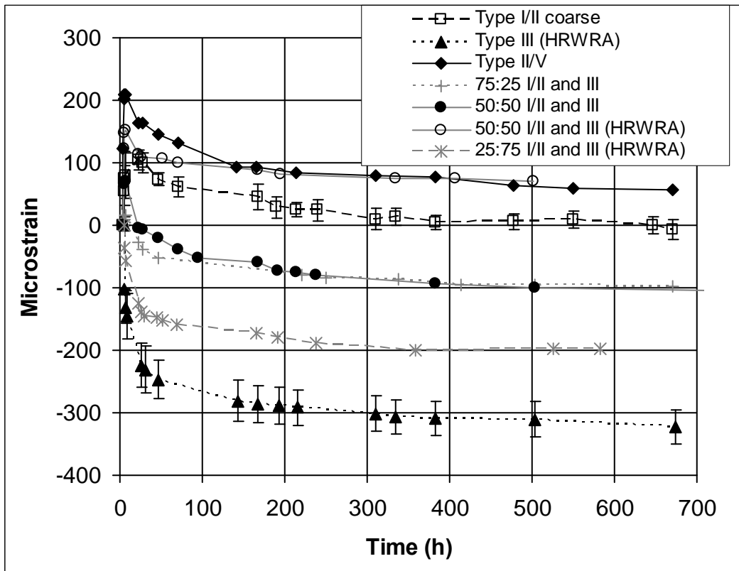
Figure 15. Autogenous deformation results for the various mortar mixtures. Error bars indicating \pm one standard deviation for three replicate specimens are provided for two of the data sets to provide some indication of variability.
