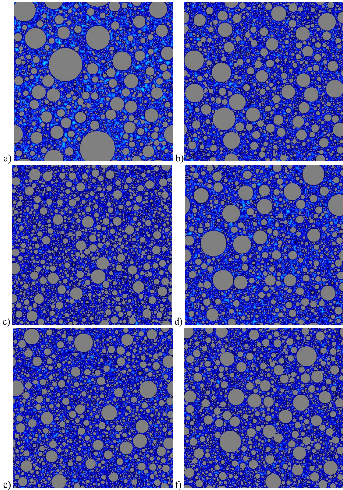
Figure 2. Two-dimensional images from simulated three-dimensional starting microstructures for pastes with w/c=0.4 and a) Type I/II, b) Type II/V, c) Type III, d) 75:25 blend of Types I/II and III, e) 50:50 blend of Types I/II and III, and f) 25:75 blend of Types I/II and III cements. Images are 200\ \mu\text{m} by 200\ \mu\text{m} ( 0.0078\ \text{in} by 0.0078\ \text{in} ).
