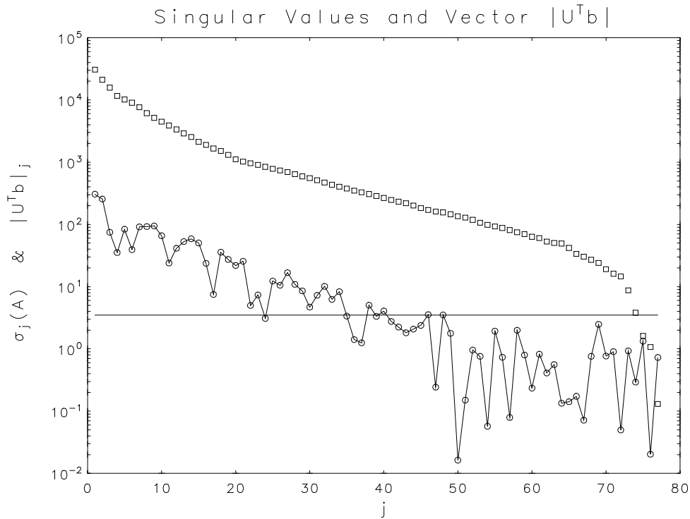
Figure 9: Singular values (squares) and first n elements of |\mathbf{U}^T \mathbf{b}| (circles) for the Burrus neutron spectrum problem. The horizontal line represents the truncation level \tau = 3.5 .
