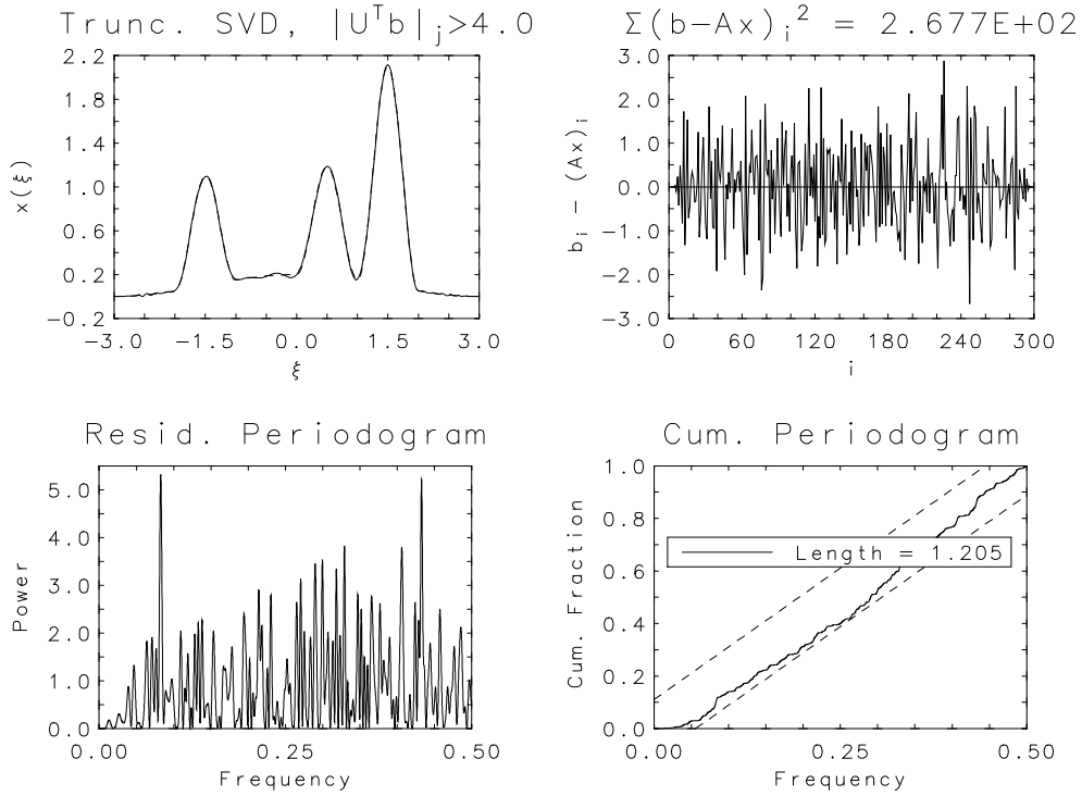
Figure 6: Truncated solution and diagnostic plots for the modified Phillips problem with \tau = 4
