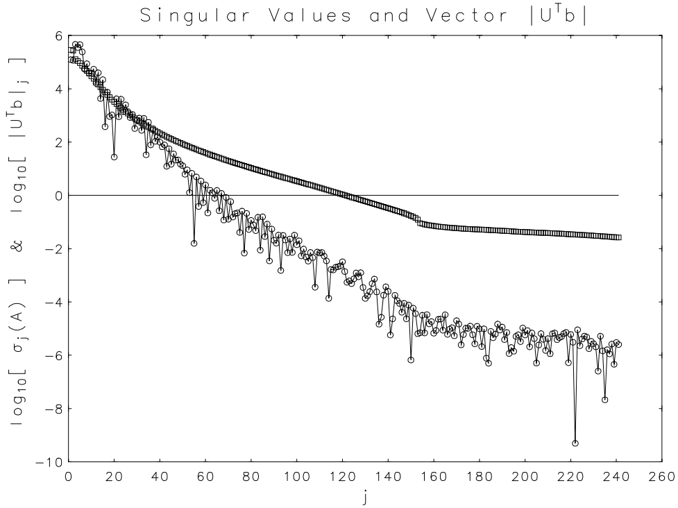
Figure 4: Singular values (squares) and first n elements of |\mathbf{U}^T \mathbf{b}| (circles) for the modified Phillips problem with no random errors
