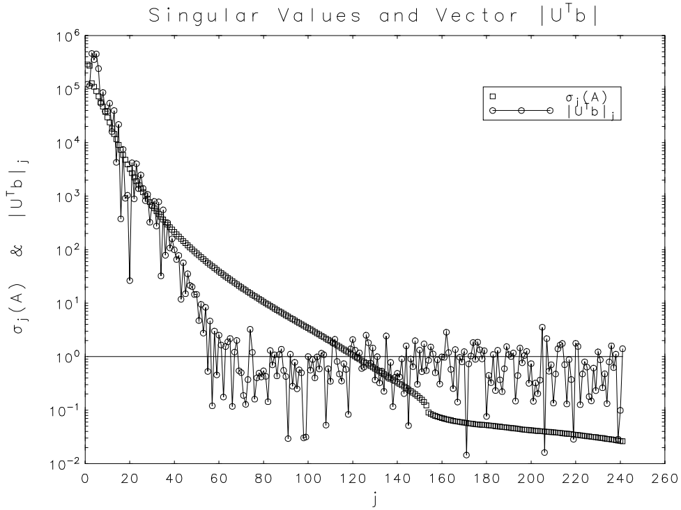
Figure 3: Singular values (squares) and first n elements of |\mathbf{U}^T \mathbf{b}| (circles) for the modified Phillips problem
