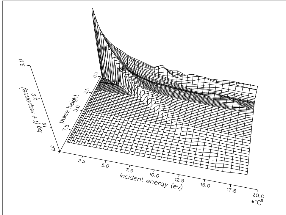
Figure 7: Instrument response functions for the Burrus neutron spectrum problem. The quantity \log_{10}[1 + K_i(E)] is plotted in order to more clearly show the structure for higher energies.
