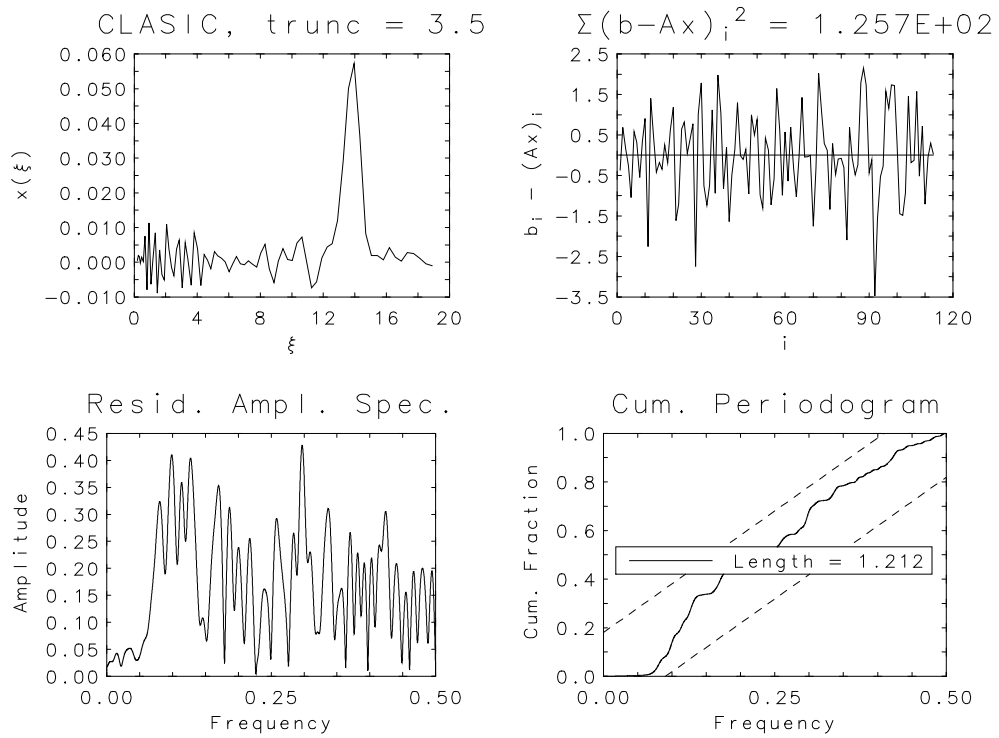
Figure 10: Truncated solution and diagnostic plots for the Burrus neutron spectrum problem with \tau = 3.5
