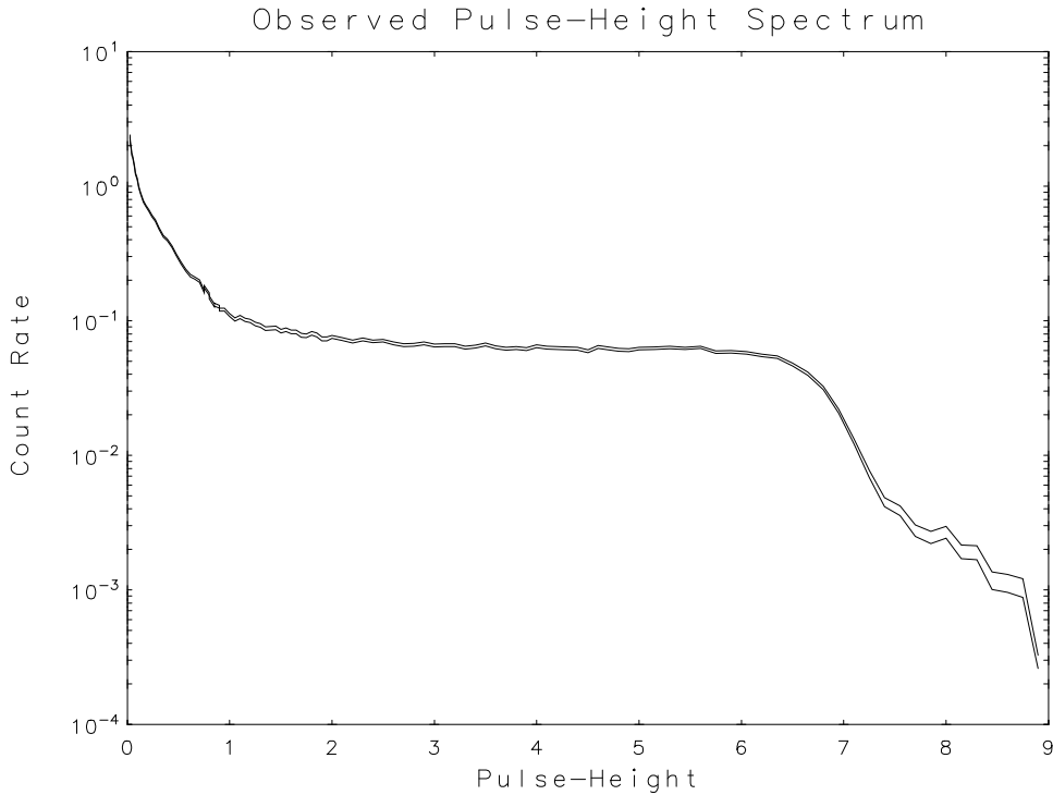
Figure 8: Measured pulse-height spectrum for the Burrus problem. The two piecewise linear curves are the \pm one standard deviation bounds for the measured values
