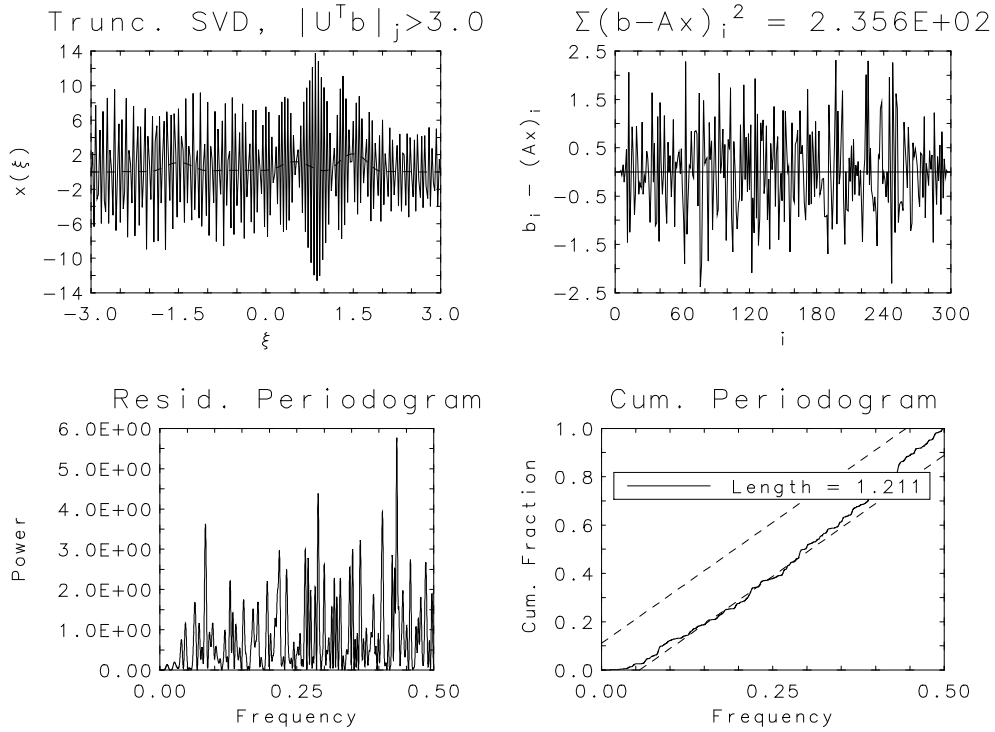
Figure 5: Truncated solution and diagnostic plots for the modified Phillips problem with \tau = 3
