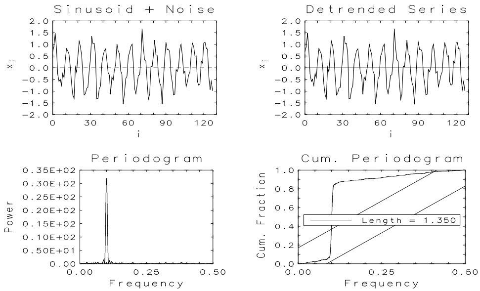
Figure 13: Periodogram and cumulative periodogram for a single sinusoid plus white noise time series
