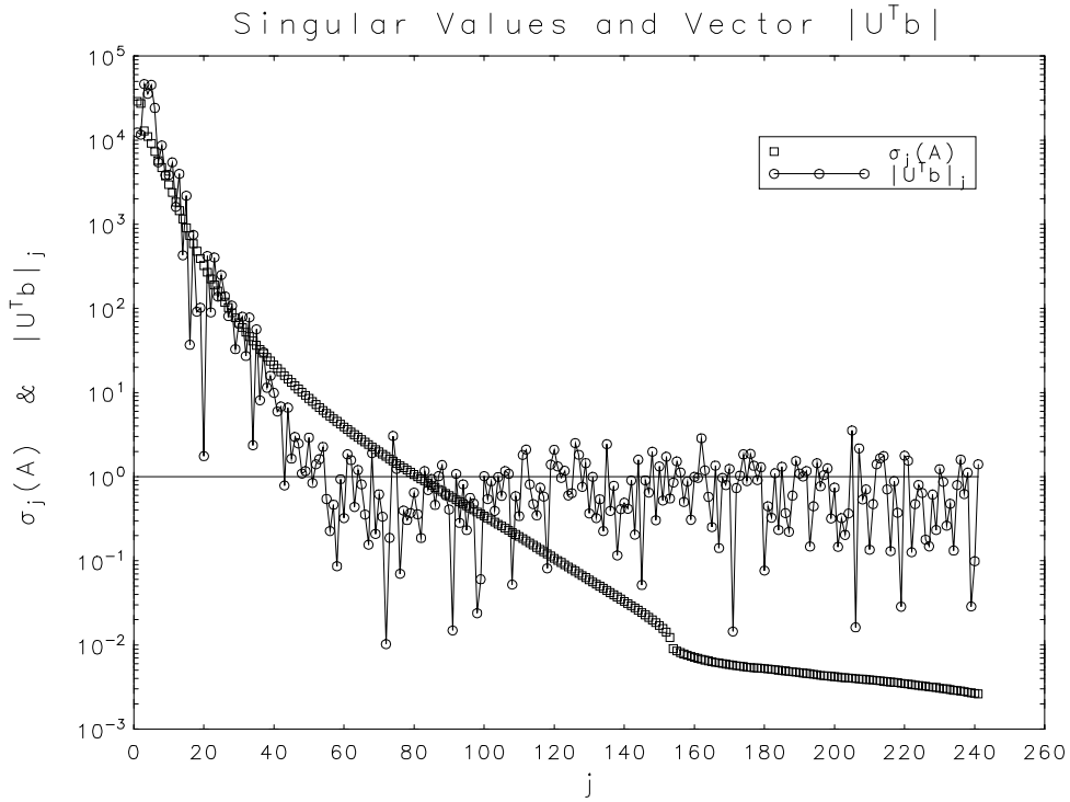
Figure 11: Singular values (squares) and first n elements of |\mathbf{U}^T \mathbf{b}| (circles) obtained by increasing the errors in the modified Phillips problem by a factor of 10
