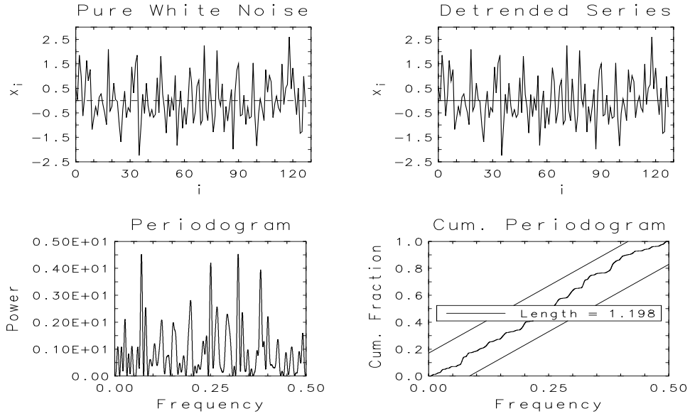
Figure 12: Periodogram and cumulative periodogram for a white noise time series
