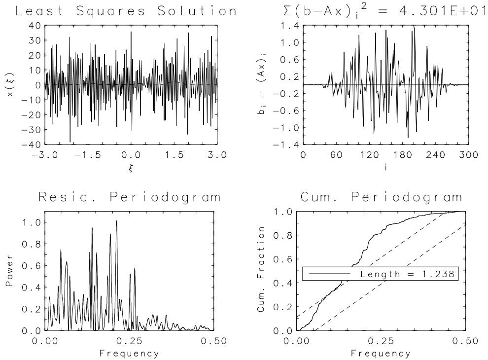
Figure 2: Least squares estimate and diagnostics for the modified Phillips problem
