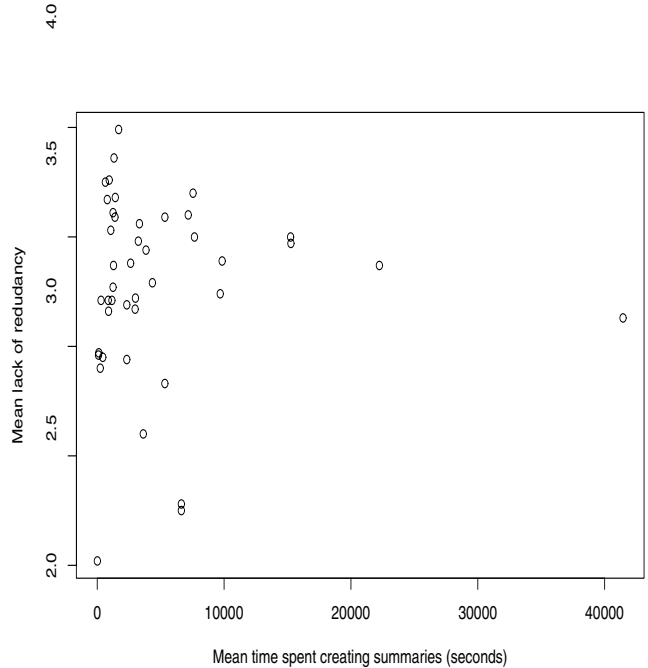
Figure 14: Summary creation time vs. lack of redundancy
