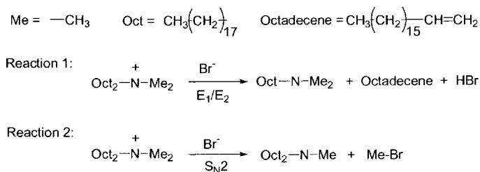
Figure 8. Proposed DMDODA-clay thermal degradation routes based on the chemical ionization MS analysis.
