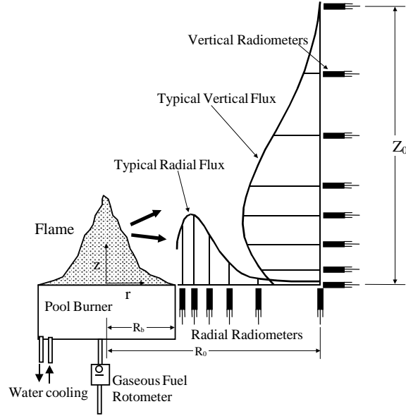
Figure 1. A schematic diagram of the set-up used to measure the radiative fraction.
