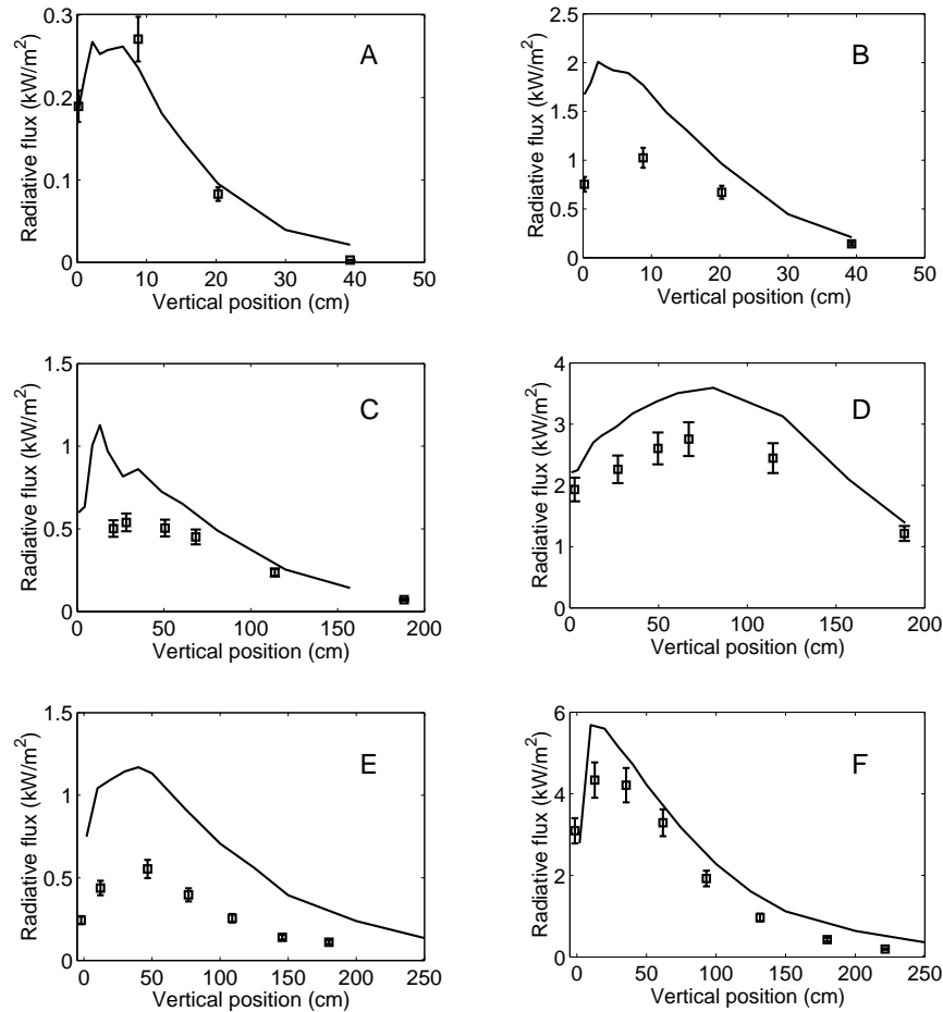
Figure 4. Comparison of the measured (squares) and predicted (lines) vertical heat flux distributions outside the methane flames. See Table 2 for the explanation of symbols A...F.
