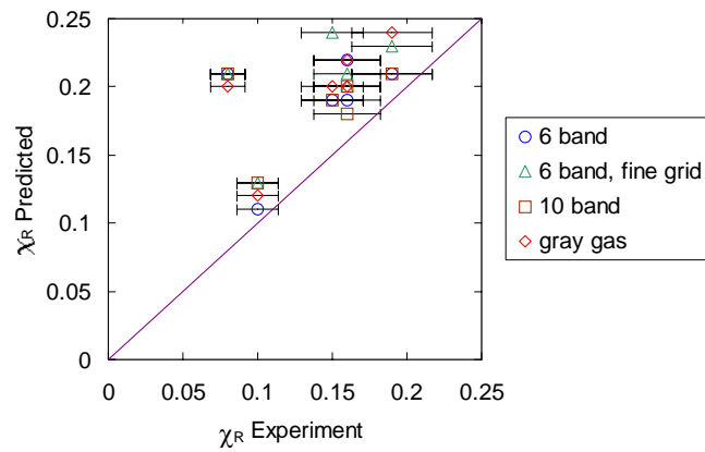
Figure 2. A summary of the accuracy of the radiative fraction prediction. The estimated uncertainty of the experimental values is 11 %.
