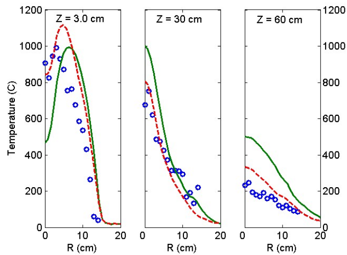
Figure 6. Comparison of the measured (circles) and predicted temperatures in the 30 cm methanol pool flame. The simulated temperatures are shown for both the predicted (solid lines) and the prescribed (dashed lines) burning rates.
