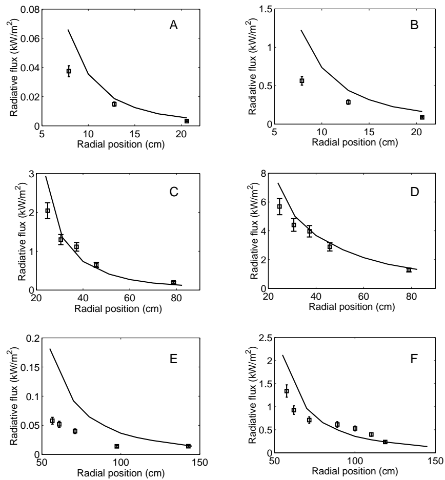
Figure 3. Comparison of the measured (squares) and predicted (lines) radial heat flux distributions outside the methane flames. See Table 2 for the explanation of symbols A...F.
