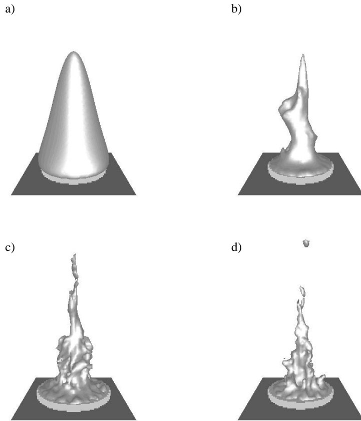
Figure 5. Instantaneous flame shapes of the simulated methanol pool fires. The diameters of the pools are a) 1.0 cm, b) 10 cm, c) 30 cm and d) 100 cm.
