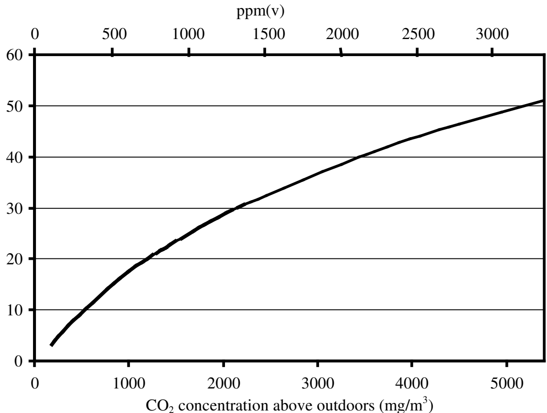
Figure 2 Percent of Visitors Dissatisfied with Bioeffluents Odor as a Function of CO 2 Concentration (CEC 1992)
