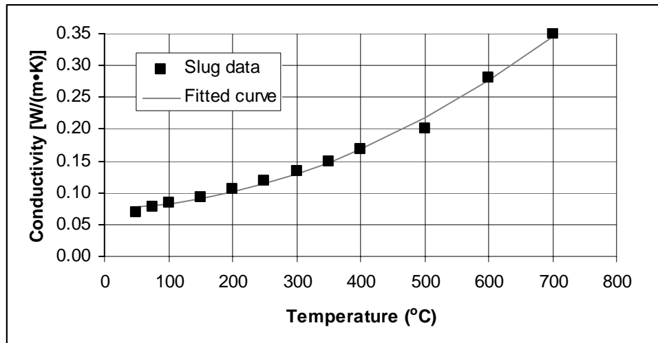
Figure 9. Measured and fitted effective thermal conductivity vs. temperature for the low density portland cement-based FRM. Fitted equation has the form: k = 0.102 - 0.00024T + (5.05 * 10^{-7})T^2 with k in units of W/(m·K) and T in K.
