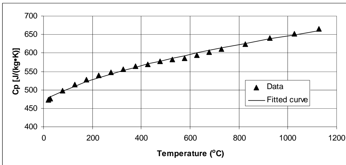
Figure 1. Literature values [12] and fitted curve for heat capacity of 304 stainless steel. Fitted curve is of the form C_p = A + BT + C\ln(T) with T in degrees K, and A=6.683, B=0.04906, and C=80.74.
