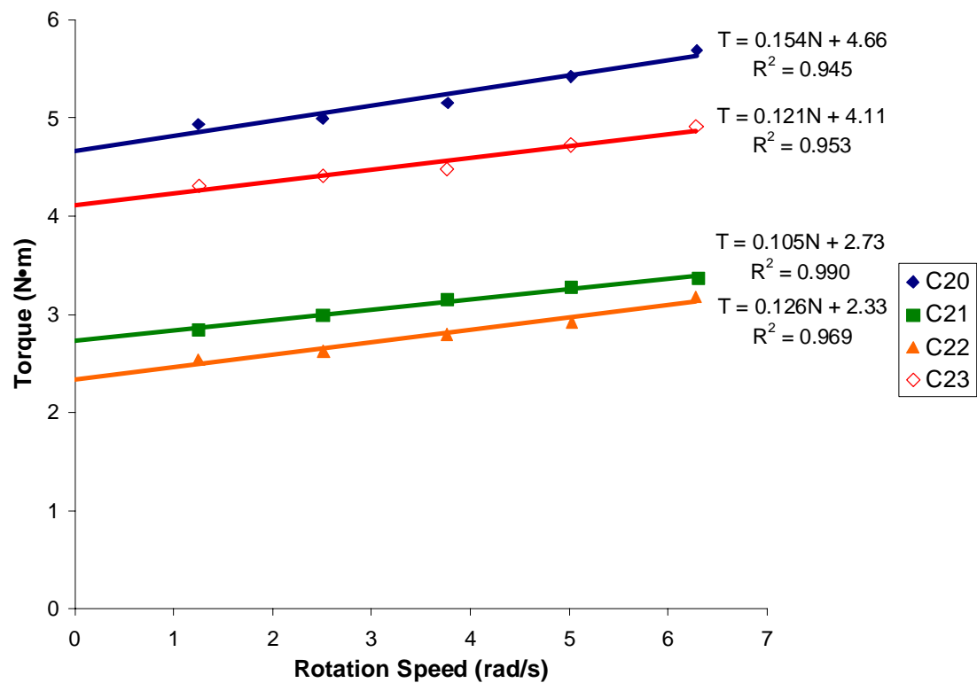
Figure 7 : Flow curves obtained with ICAR rheometer for Series 2 (C20 to C23)
