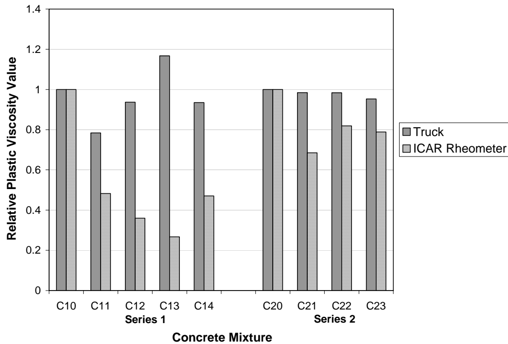
Figure 9 : Relative plastic viscosity, as defined by the ratio of the measured plastic viscosity with the control mixture plastic viscosity, recorded by the mixing truck and ICAR rheometer. The control mixtures are C10 and C20.
