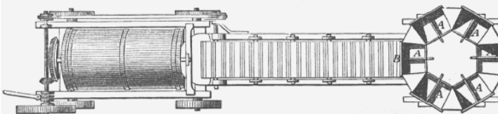
Fig. 109. Le Messurier's Concrete Machine. Elevation.
