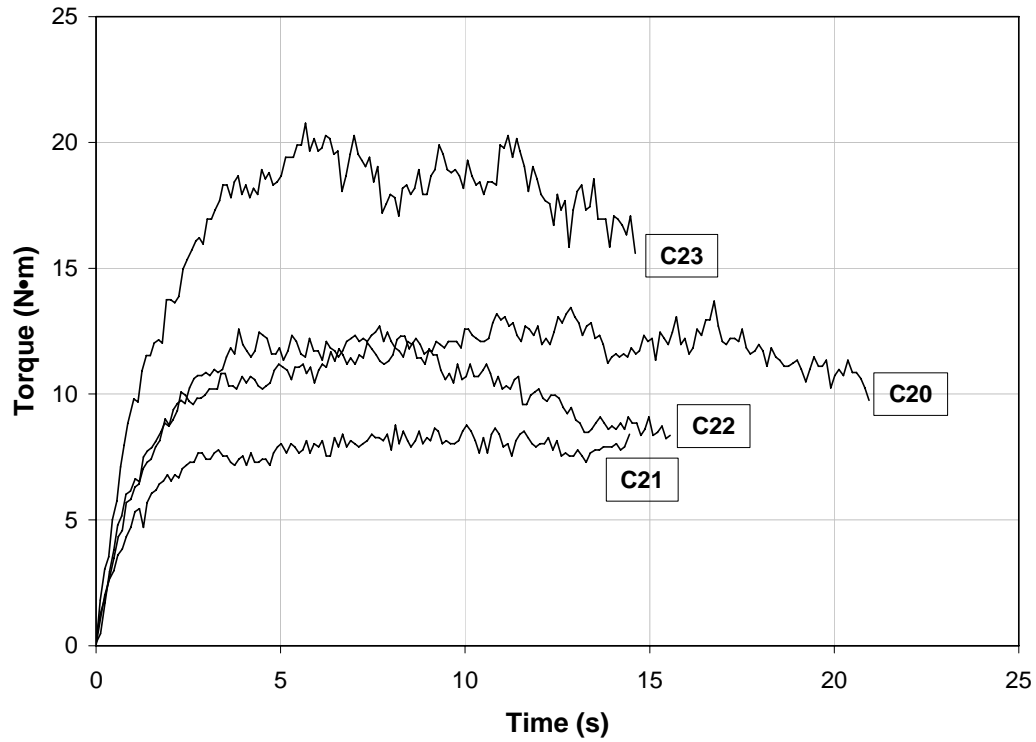
Figure 8: Typical ICAR rheometer stress growth test results for selected mixtures
