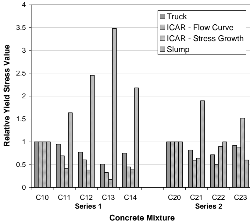
Figure 12: Relative yield values, as defined by the ratio of the measured yield stress with the control mixture yield stress, as recorded by mixing truck, ICAR rheometer, and slump test. The control mixtures are C10 and C20.
