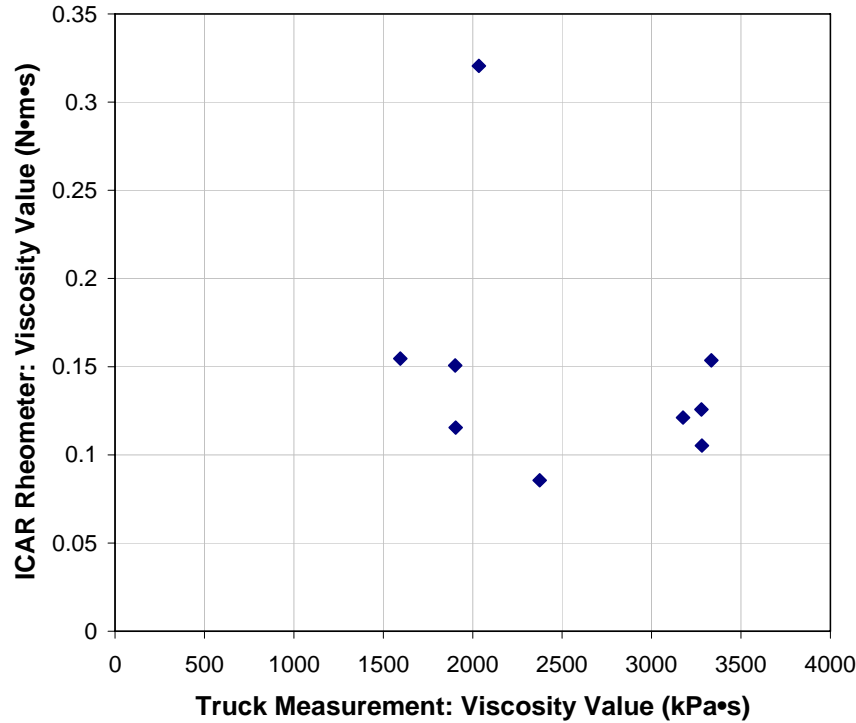
Figure 11: Correlation of plastic viscosity value between ICAR rheometer and truck
