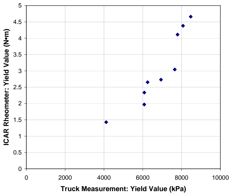
Figure 13: Correlation of yield value between ICAR rheometer and truck
