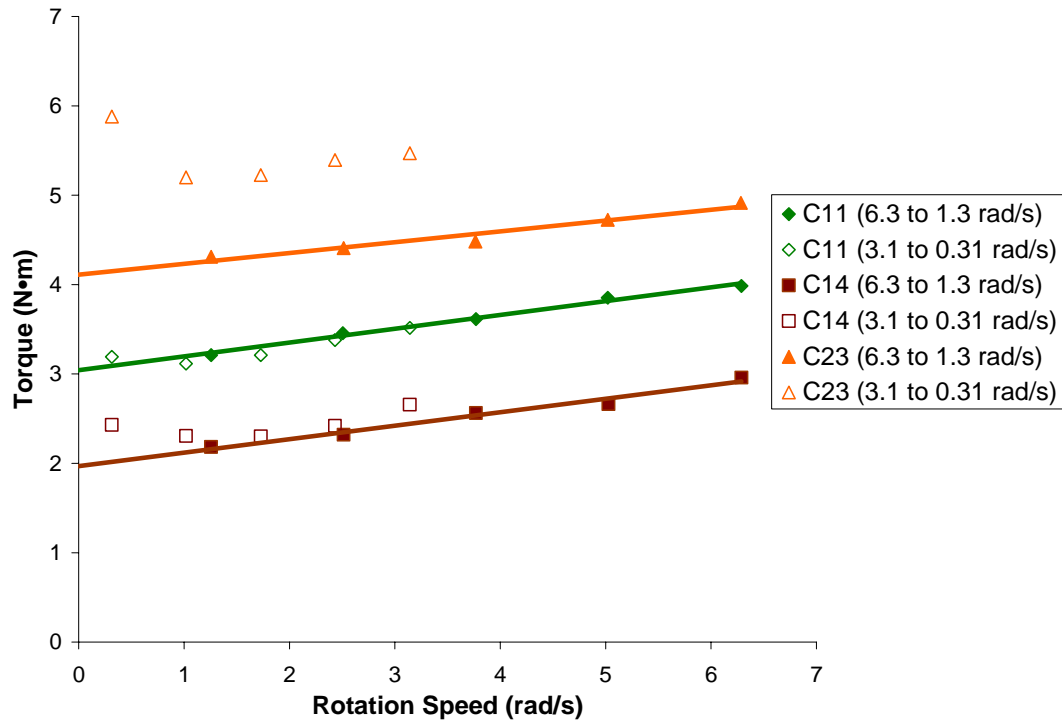
Figure 10: Illustration of slope of the flow curves for selected ICAR rheometer measurements
