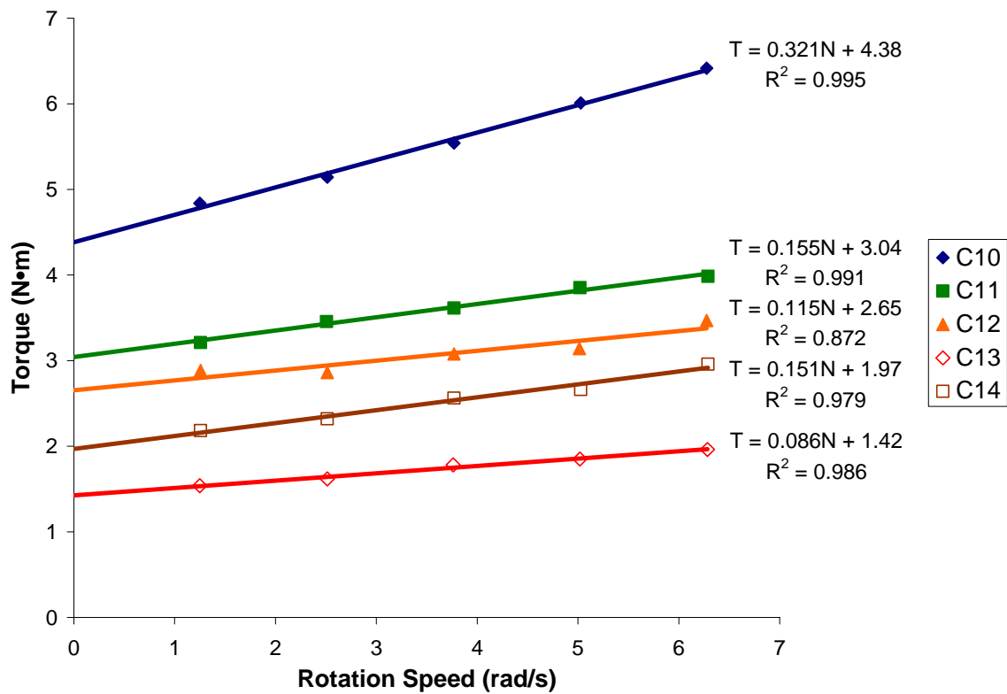
Figure 6 : Flow curves obtained with ICAR rheometer for Series 1 (C10 to C14)
