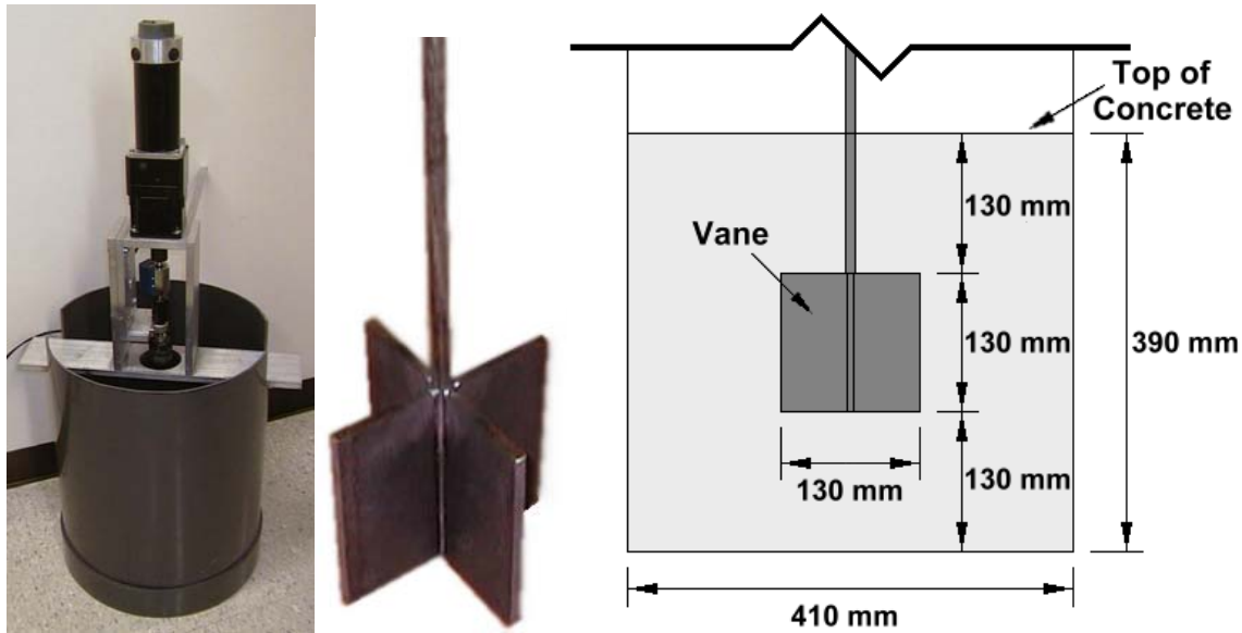
Figure 3 : View of the ICAR rheometer prototype, vane, and principal dimensions
