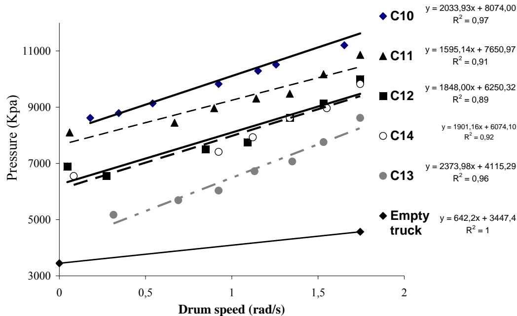
Figure 4: Flow curves obtained with the truck mixer (empty truck, C10 to C14 mixture)
