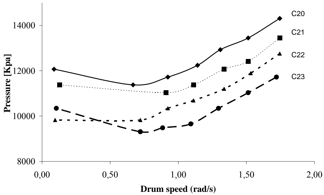
Figure 5: Flow curves obtained with the truck mixer (C20 to C23 mixture)
