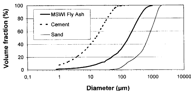
Fig. 1. Size grading curves of cement, MSWI fly ash and sand.
