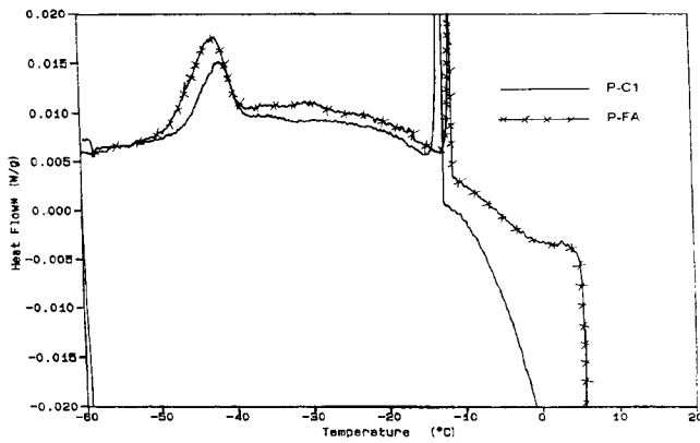
Fig. 5. DSC curves obtained for the P-C1 and P-FA pastes after successive immersions.
