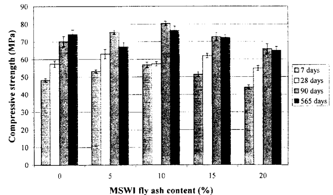
Fig. 8. Compressive strengths of the M0, M5, M10, M15 and M20 mortars after 7, 28, 90 and 565 days.
