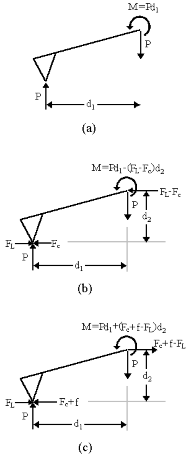
Figure 2 Free-body diagrams of the AFM cantilever probe for (a) a normal force, P , applied to the probe tip (idealized indentation), (b) forces applied during indentation testing, and (c) forces applied during nanoscratch testing with a scratch angle of 0^\circ .
