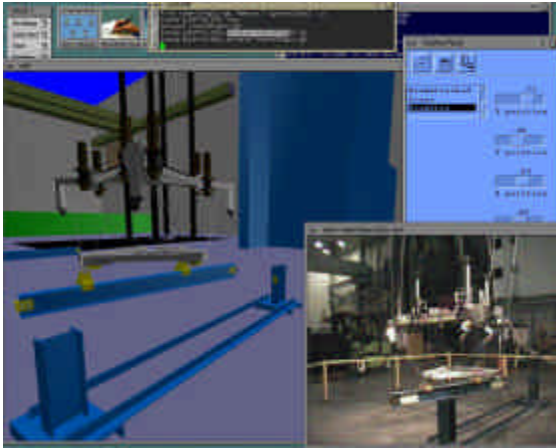
Fig. 1: 3-D visualization of a robotic crane during an assembly operation with a steel I-beam. The inset video image shows the correspondence between the model and the real system. The real-time data driving the visualization subsystem came from TETRA's real-time controller, via the tetSock proto-protocol.
