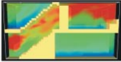
Computer simulation of the Cherry Road fire.
