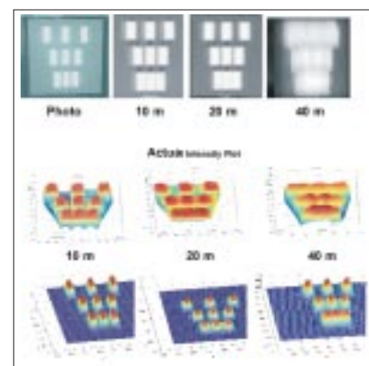
Intensity plots of retroreflective bar codes.
