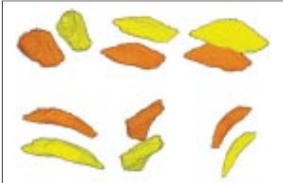
Six views, from various rotation angles, of a real aggregate particle taken from an x-ray tomographic image (orange), and the same particle, re-created using spherical harmonic analysis (yellow). The mathematical analysis correctly captures the real three-dimensional shape of the irregular aggregate particle.
