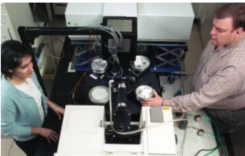
Dr. Christopher White and Ms. Mona Anaraki, a student, are working on the high-throughput analysis device for characterizing optical, chemical and physical degradation changes in polymeric construction materials. At present, the device can automatically make 9 analytical measurements on each of 70 specimens in one hour. This data is then automatically and electronically downloaded to an informatics system for further analysis.
