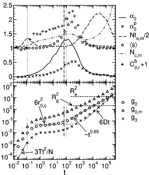
FIG. 16. Recapitulating the comparison of the time dependence of various quantities discussed in this paper. In all cases, the temperature is T=0.46 ( T_{MCT} \approx 0.45 ). The upper figure shows the non-Gaussian parameters \alpha_2 and \alpha_2^p . These quantities are averages over all monomers and all chains in the melt. The other quantities shown are calculated from the 6.5% of highly mobile monomers. They are: the fraction of mobile end-monomers Nf_{e,m}/2 , the average string length \langle s \rangle , the average length of mobile contiguous segments of a chain N_{c,m} , and the cosine of the angle between the displacement of a mobile monomer and the vector to one of its nearest mobile neighbors in the chain C_{d,r}^b . The vertical dotted lines indicate the time of the first peak of Nf_{e,m}/2 ( t=0.1104 ), the time t_{\alpha_2}^* ( =100.894 ) where \alpha_2 is maximum, whereas the vertical dashed line indicates the time t_{clu}^{max} when the clusters formed by the subset of mobile monomers is largest for T=0.46 ( t_{clu}^{max}=65.85 ) (Ref. 25). These times are also included in the lower figure (vertical dotted resp. dashed lines). This figure shows the MSD of all monomers g_0 , of the mobile monomers g_{0,m} , and of the center-of-mass g_3 . The behavior in the ballistic ( \sim t^2 ), the subdiffusive ( \sim t^{0.65} ) and the diffusive regimes ( \sim t ) are indicated by solid lines. The horizontal dashed lines depict 6r_{0,c}^2 (Lindemann localization length r_{0,c} \approx 0.095 for g_0 ), the radius of gyration R_g^2 ( =2.09 ), and the end-to-end distance R_e^2 ( =12.3 ).
