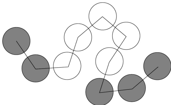
FIG. 4. A schematic diagram showing how the average length of contiguous segments of mobile monomers, N_{c,m}(t_\mu) , is defined. Assume that, at time t_\mu , only the shaded monomers are considered to be mobile. The first two monomers constitute a contiguous segment of length 2, then there are five nonmobile monomers, followed by another contiguous segment of length 3. So, the average length of contiguous mobile segments is N_{c,m}(t_\mu) = 2.5 .
