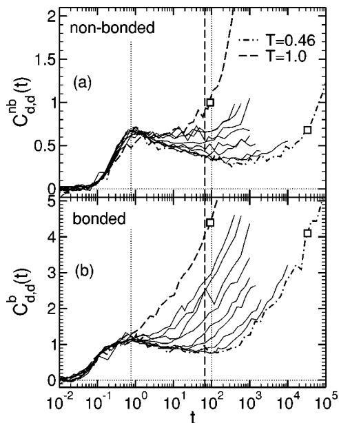
FIG. 15. C_{d,d}(t) vs time for all T . C_{d,d} measures the tendency of two neighboring mobile particles to follow each other at time t [Eq. (20)]. (a) and (b) present the results for nonbonded and bonded nearest neighbors. In both panels, the vertical dotted lines indicate the times t_{\alpha_2}^* for T=1 ( t_{\alpha_2}^*=0.766 ) and for T=0.46 ( t_{\alpha_2}^*=100.894 ), whereas the open squares mark the times when g_e/g_0 reaches its second maximum ( t \approx 92 for T=1 , t \approx 33361 for T=0.46 ; see Fig. 6). The dashed vertical line in both panels indicates the time t_{clu}^{max} when mean cluster size, calculated in Ref. 25, is maximum for T=0.46 ( t_{clu}^{max}=65.85 ). The following temperatures are shown (curves from left to right): T=1, 0.7, 0.65, 0.6, 0.55, 0.52, 0.5, 0.48, 0.47, 0.46 .
