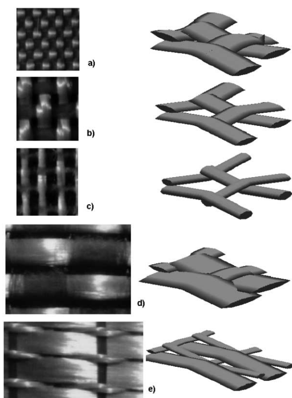
Fig. 4. Photographs (left) and computed images (right) of different types of 2D glass reinforcements: (a–c) glass multi-filaments, different weave density; (d) glass rovings; (e) unidirectional weave.
