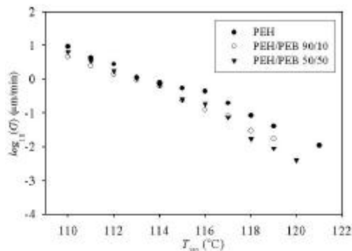
Figure 3. Spherulitic growth rates in PEH, H90 and H50 blends as a function of the isothermal temperatures.
