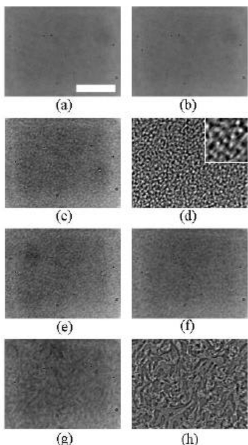
Figure 4. Optical micrographs with the double quench measurement of H40. (a) 160 °C, (b) 130 °C, (c) 130 °C for 300 min, (d) room temperature from (c), (e) 130 °C from (d), (f) 219 min from (e), (g) 938 min from (e), (h) room temperature from (g). Scale bar in (a) represents 40 \mu\text{m} .
