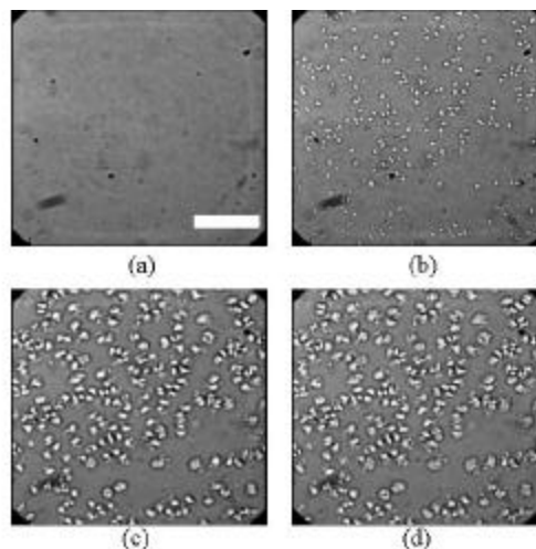
Figure 2. Optical micrographs of H50 isothermally crystallized at 117 °C. (a) 0 min, (b) 30 min, (c) 150 min, (d) 249 min. Scale bar in (a) represents 40 \mu\text{m} .
