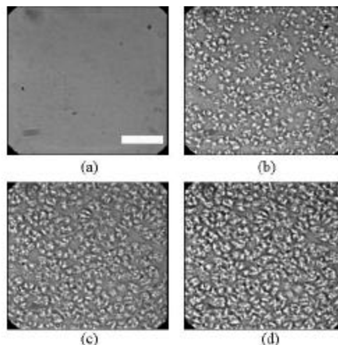
Figure 1. Optical micrographs of PEH isothermally crystallized at 117 °C. (a) 0 min, (b) 48 min, (c) 79 min, (d) 119 min. Scale bar represents 40 \mu\text{m} .
