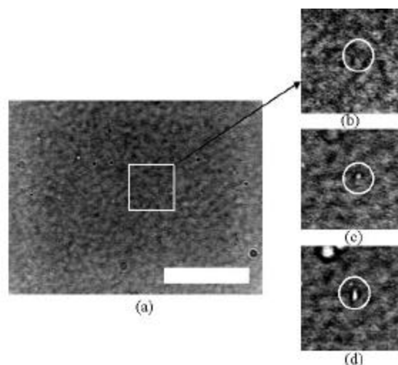
Figure 5. Optical micrographs with the double quench measurement of H40, phase separated at 130 °C for 10h first and then isothermally crystallized at 116 °C. (a) 0 min, (b) magnified enclosed part in (a) 0 min, (c) 3 min, (d) 6 min. Scale bar in (a) represents 40 \mu\text{m} .
