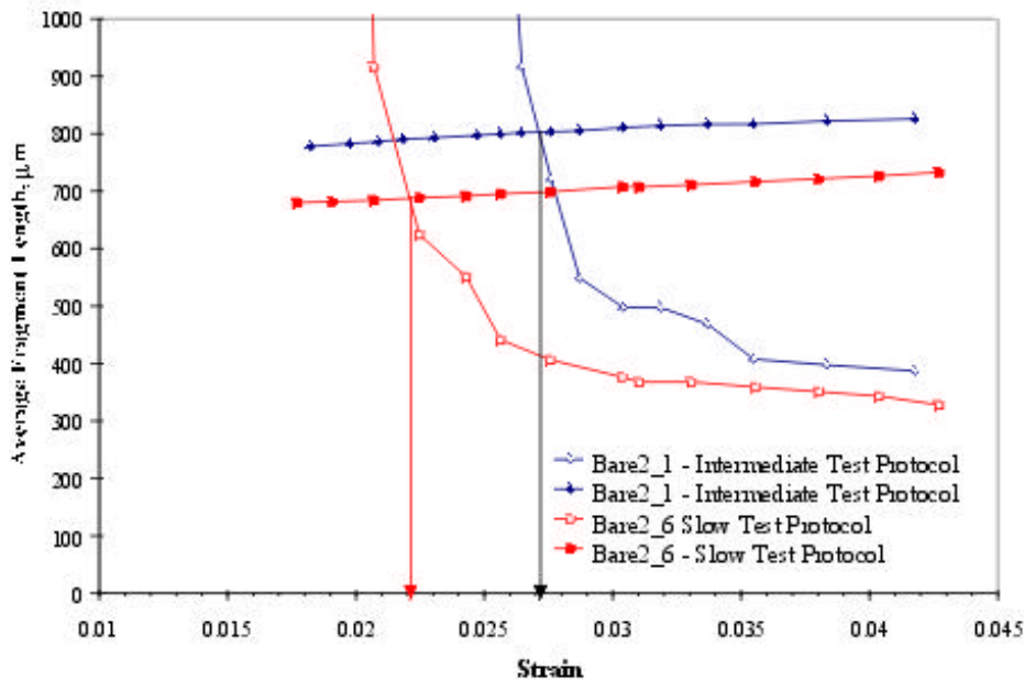
Figure 6. Graphical Determination of the 'in situ' Fiber Strength at Saturation from SFC Test Data.
