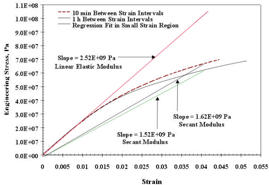
Figure 5. Typical Stress-Strain Plots from 10 min. and 1 h Test Protocol Specimens.
