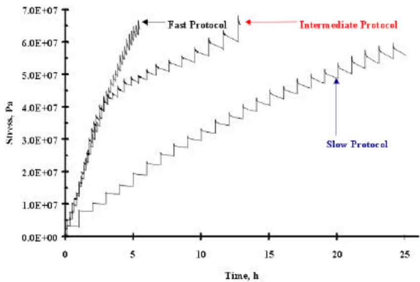
Figure 3. Stress-Time Curves for Test Protocols.
