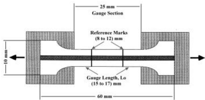
Figure 2. Typical Specimen Dimensions.
