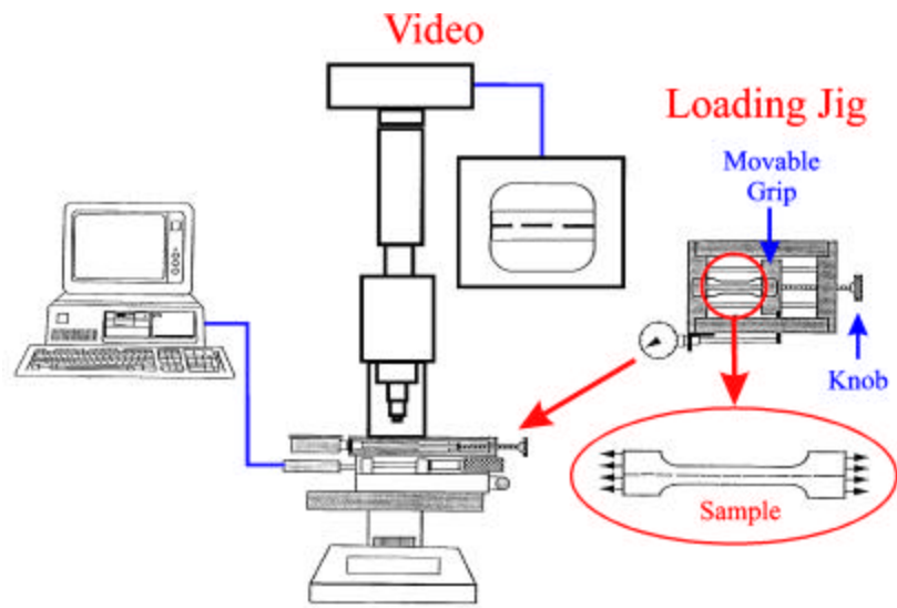
Figure 1. Schematic of Testing Apparatus.
