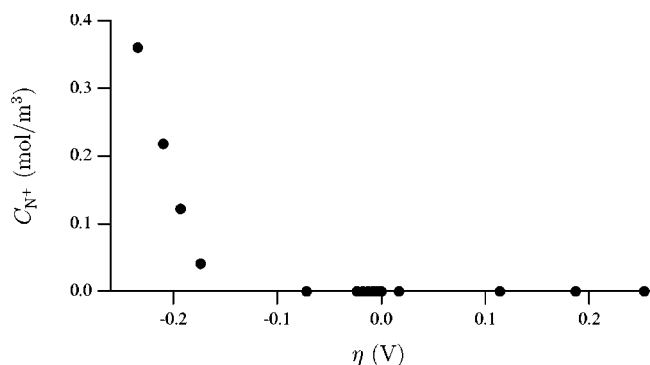
FIG. 7. Concentration C_{N^+} of N^+ in the deposited electrode as a function of overpotential \eta .
