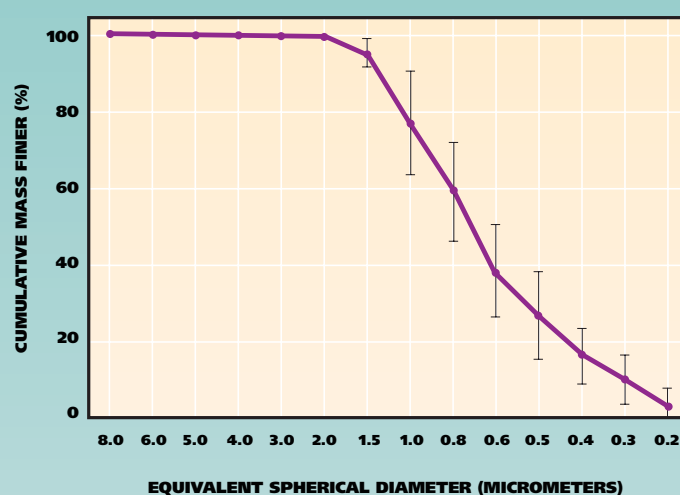
Figure 6. Representative particle size distributions of unmilled zirconia-hybridized amorphous calcium phosphate (Zr-ACP) (A) and milled Zr-ACP (B).
