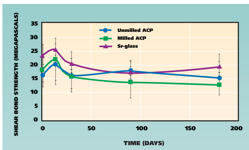
Figure 8. Effect of filler type on the shear bond strength of bisphenol glycidylmethacrylate, triethyleneglycol dimethacrylate, 2-hydroxyethyl methacrylate, zirconyl dimethacrylate-based composites aged in distilled water at 37°C. The values are mean \pm standard deviation of the minimum of seven specimens in each experimental group. ACP: Amorphous calcium phosphate. Sr-glass: Strontium glass.
