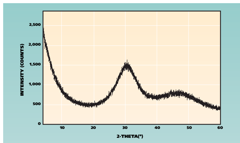
Figure 4. X-ray diffraction pattern.
