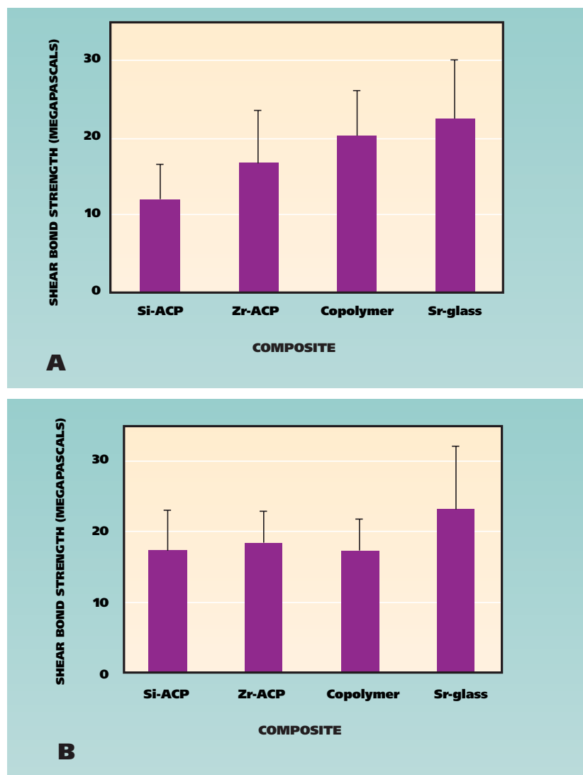
Figure 7. Mean group 24-hour shear bond strength data obtained with triethyleneglycol dimethacrylate, pyromellitic glycerol dimethacrylate resin ( A ) and bisphenol glycidylmethacrylate, triethyleneglycol dimethacrylate, 2 hydroxyethylmethacrylate, zirconyl dimethacrylate resin ( B ) basing-composites filled with silica-hybridized amorphous calcium phosphate (Si-ACP) and zirconia-hybridized amorphous calcium (Zr-ACP) compared with unfilled copolymer and strontium glass–(Sr-glass–) filled composites. The number of specimens per group was eight or more.
