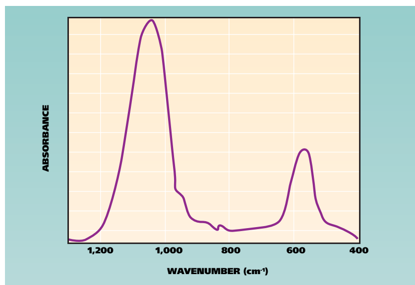
Figure 5. Fournier transformed infrared spectrum. \text{cm}^{-1} : Inverse centimeters.
