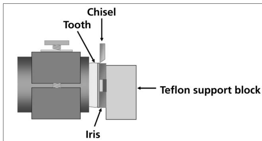
Figure 3. Shear bond strength testing assembly. Teflon is a polytetrafluoroethylene manufactured by DuPont, Wilmington, Del.
