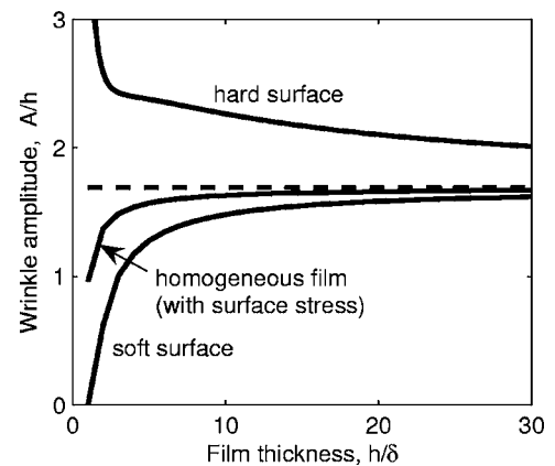
Fig. 3. Wrinkle amplitude as a function of film thickness subjected to a constant strain ( \varepsilon = -0.02 ), for a homogeneous film ( \bar{E}_f/\bar{E}_s=1,000 , f=10\bar{E}_s\delta ) in comparison with bilayer films with a soft surface ( \bar{E}_f^*/\bar{E}_f=0.1 ) and a hard surface ( \bar{E}_f^*/\bar{E}_f=10 ), respectively. The dashed line corresponds to a homogeneous film with no surface stress effect ( f=0 ).
