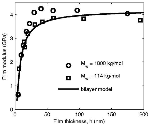
Fig. 8. Effective modulus as a function of film thickness for PS films
