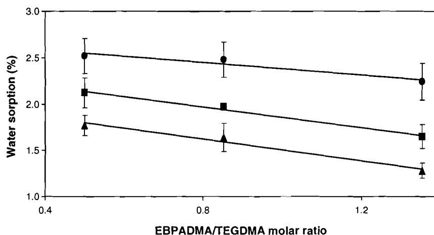
Fig. 7. Functional dependence between the maximum WS (mean \pm SD (indicated by bars)) and the molar ratio of EBPADMA/TEGDMA in the resin for ETHM copolymers (▲), unmilled ACP/ETHM composites (●) and milled ACP/ETHM composites (■).
