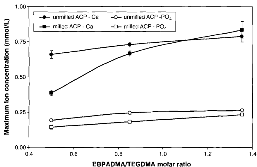
Fig. 6. Functional dependence between the maximum concentration of the release calcium and phosphate ions (mean \pm SD (indicated by bars)) and the molar ratio of EBPADMA/TEGDMA in the resin.
