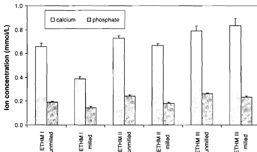
Fig. 3. Maximum concentration of the mineral ions (mean \pm SD (indicated by bars)) released from ETHMI, ETHMII and ETHMIII resin composites filled with unmilled or milled Zr-ACP after 720 h of immersion in buffered saline. The SD is taken as a measure of the standard uncertainty; n \geq 3 .
