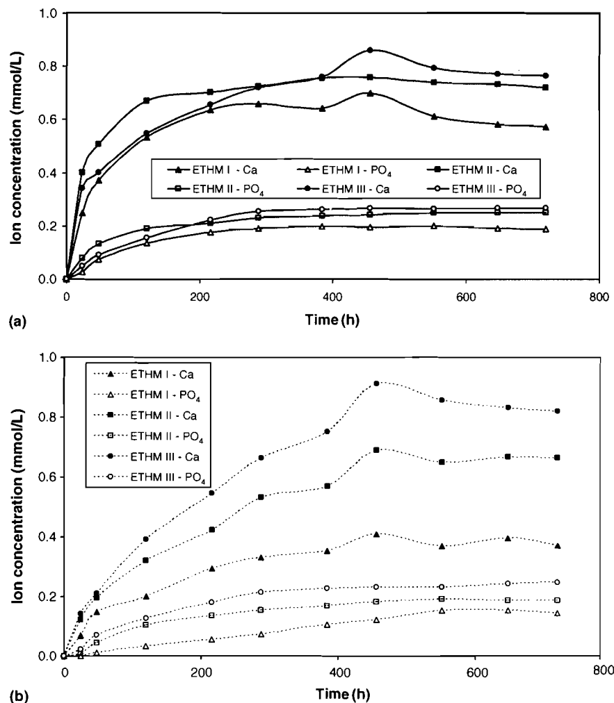
Fig. 2. Ion release kinetic profiles of unmilld ACP (a) and milled ACP (b) composites. SDs of the reported values ranged from 0.005 mmol/L to 0.011 mmol/L and from 0.003 mmol/L to 0.009 mmol/L for calcium and phosphate, respectively; n \geq 3 .
