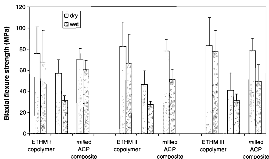
Fig. 5. Biaxial flexure strength (mean \pm SD (indicated by bars)) of dry and wet ETHMI, ETHMII and ETHMIII copolymers and their unmilled or milled Zr-ACP composites. The number of runs in each experimental group n \geq 5 . Standard deviation (SD) is taken as a measure of the standard uncertainty; n \geq 5 .
