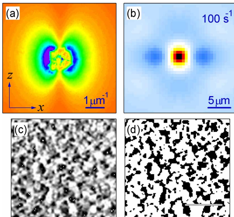
Fig. 10. Combined optical measurements of shear-induced macrostructure ( \dot{\gamma} = 100 \text{ s}^{-1} , PEO2–LRD3) in the x - z plane. Image (a) is the small-angle light-scattering pattern, S(\mathbf{q}) . Image (c) is a corresponding real-space micrograph, which yields a map (d) (scale bar = 25 \mu\text{m} ) of \psi(\mathbf{r}) , the local composition of gel-like domains. Image (b) is the two-point composition correlation function, c(\mathbf{r}) , computed from \psi(\mathbf{r}) .
