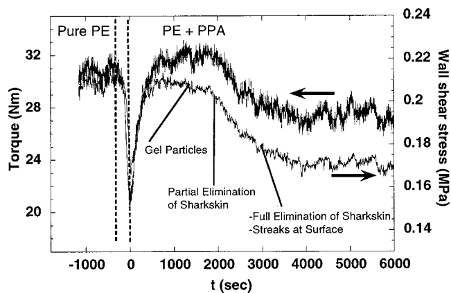
FIG. 6. Evolution of the pressure and torque in the extruder system upon addition of the polymer processing additive.
