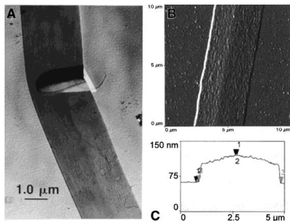
Figure 3. Morphology of individual L. arizonica silk ribbons from a community web: (A) Bright-field TEM of individual ribbon on carbon substrate shadowed with W/Ta, 2.5\ \mu\text{m} wide. (B) Noncontact AFM image of ribbon on glass substrate, uncoated. (C) Line scan of AFM image in Figure 3B to measure approximate ribbon thickness (40–50 nm); see text.
