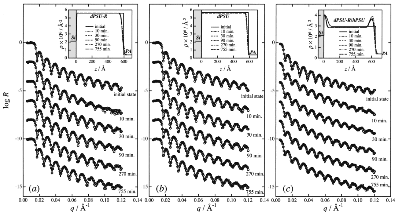
Figure 2. Neutron reflectivity profiles for different annealing times: experimental profiles (○) and the best-fit profiles (—) with the corresponding scattering length density profiles provided as insets. All measurements were performed with the neutron beam entering through the silicon wafer. Key: (a) pure reactive system, Si/dPSU-R//PA//air; (b) pure nonreactive system Si//dPSU//PA//air; (c) diluted reactive system Si//hPSU/dPSU-R//PA//air.
