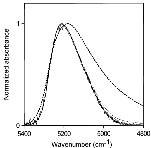
Fig. 12. Normalized NIR spectra of up to 4 mL water in 50 mL acetic acid (water concentrations of 0.056 mol/L to 4.44 mol/L water). The normalized spectrum of liquid water is shown as a dotted line.
