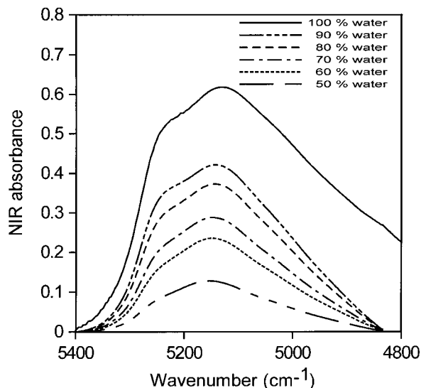
Fig. 16. Subtracted spectra: the spectrum of 40 % volume fraction of water in acetone was subtracted from the spectra of 50 %, 60 %, 70 %, 80 %, and 90 % volume fraction of water in acetone and from the spectrum of pure water.
