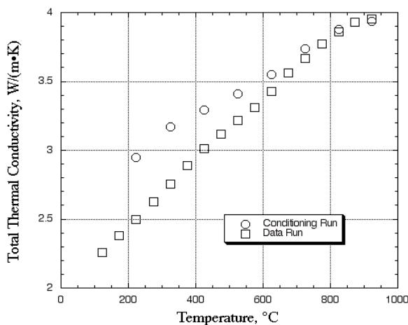
Fig. 1. Raw thermal conductivity data for one of the 350 \mu\text{m} thick coated specimens after polishing to 0.7 \mu\text{m} average surface roughness.
