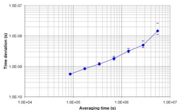
Figure 7. Time deviation of NIST-NRC link for the period from January through August, 2007.
