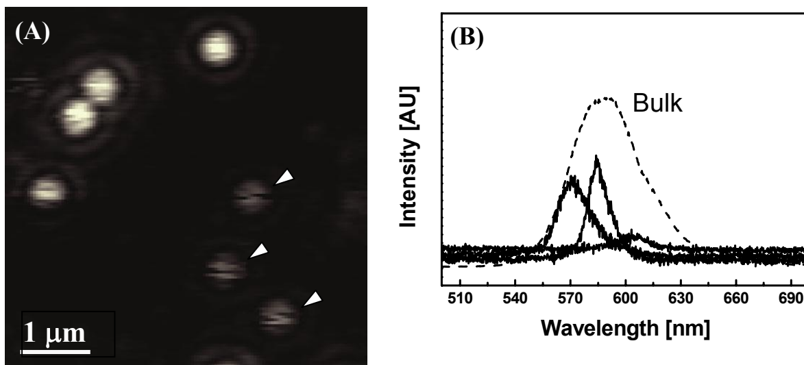
Figure 2. (A) A typical confocal fluorescence micrograph of MDA-QDs spin-cast on a glass coverslip. Four bright spots at the top left corner of the image are clusters of 2 to 3 single QDs, and the three dimmer spots indicated with arrows are from single MDA-QDs. (B) A Spectrum of an ensemble of QDs in solution and several single QD emission spectra are shown to demonstrate the spectral diversity of single QDs in the ensemble.
