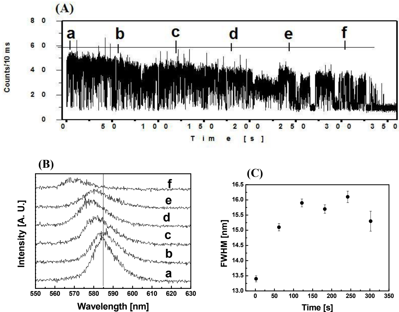
Figure 3. (A) Fluorescence intermittency from a single MDA-conjugated CdSe/ZnS QD under continuous illumination as a function of time. (B) Time-dependent spectral shift of a single QD. The time points at which each spectrum was collected are shown in (A) with indices (a) to (f). One of the single QDs marked with arrows in Fig. 2 (A) was continuously exposed to a laser spot and the data were collected with a total integration time of 5 seconds for each spectrum. (C) Full width of the half maximum of the emission peak. The error bars represent one standard deviations from the Gaussian fittings.
