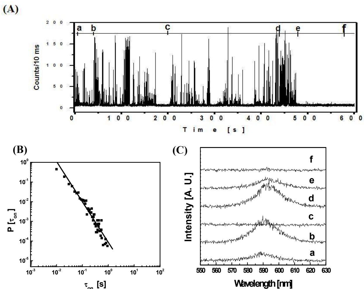
Figure 4. (A) Fluorescence intermittency from a single AMDNA-conjugated CdSe/ZnS MDA-QD under continuous illumination as a function of time. (B) Log-log weighted probability density plots of the light-emitting episodes for a single AMDNA-QD. The data was fit to a power law with an exponent of 2.06 \pm 0.08 . (C) Illumination-time-dependent spectral shift of a single QD. The time points for each spectrum collected are shown in (A) with indices (a) to (f).
